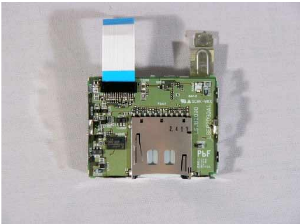
SD Card Unit PCB (Bottom view)
