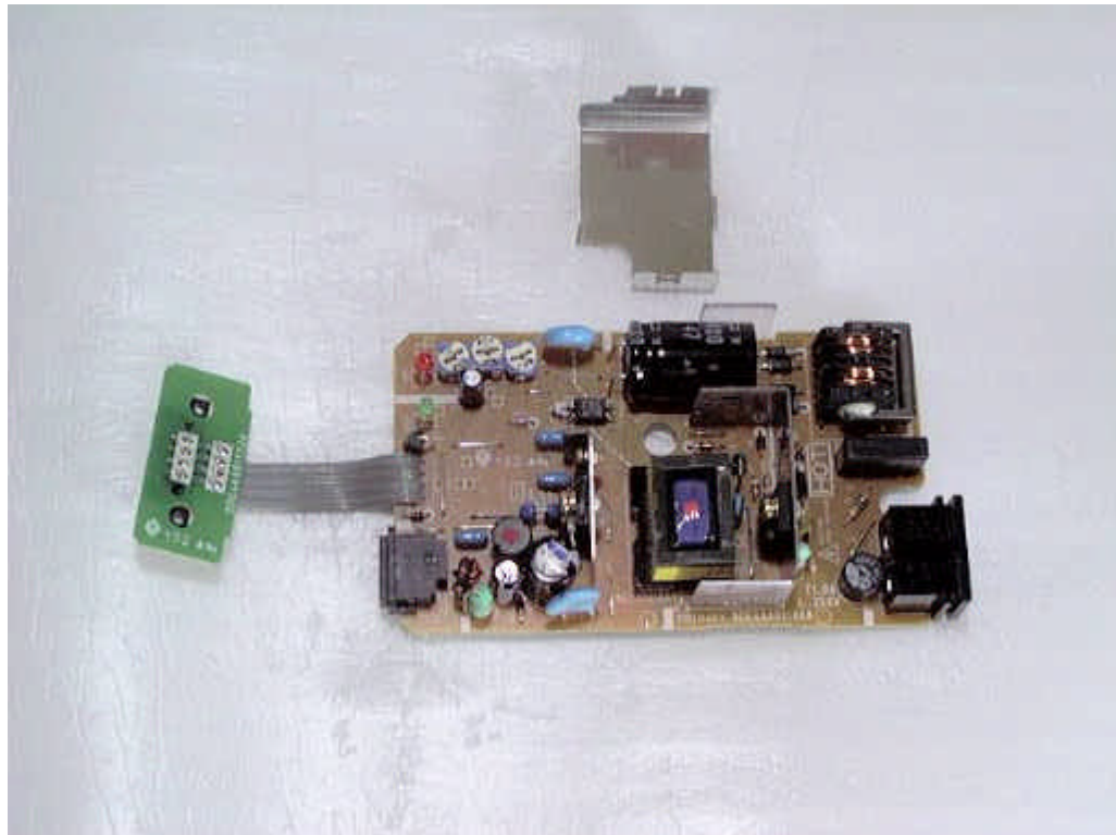
AC Adaptor PCB (Top view)
