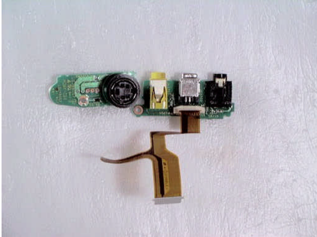
Jack PCB (Top view)
