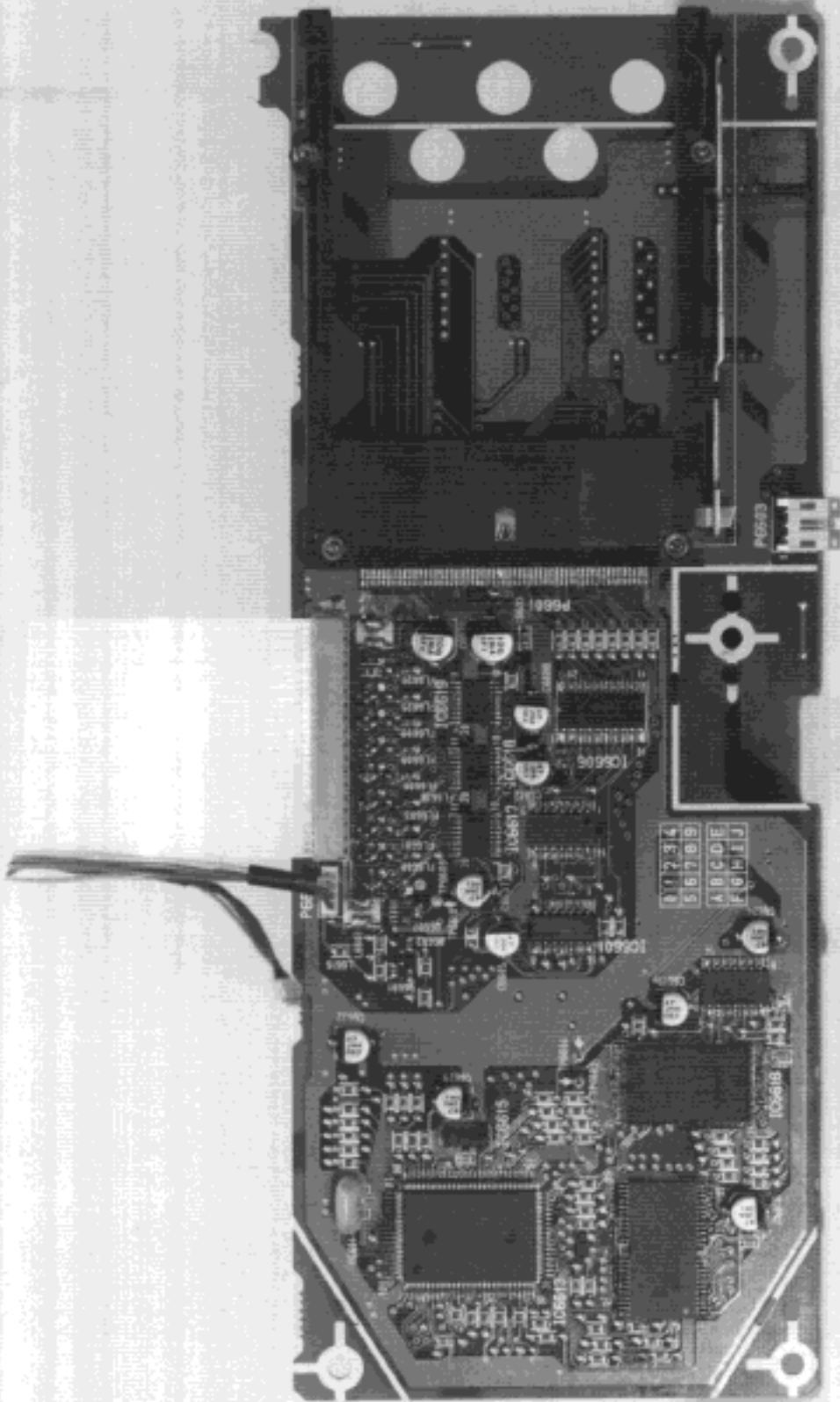
SVGA 2 CARD PCB (TOP VIEW)
