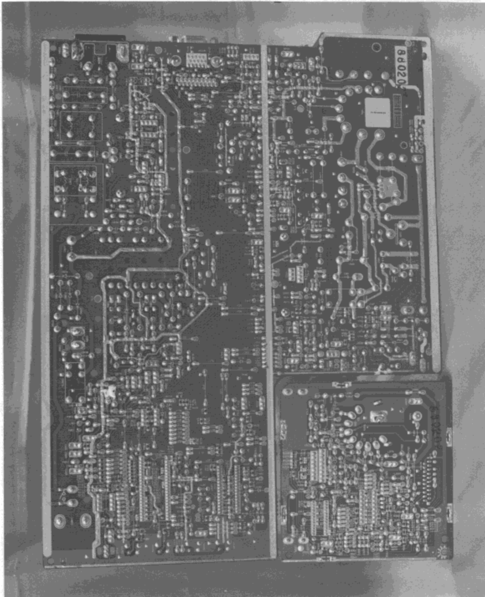
Fig 5. Main & CRT PWB, Foil Side
