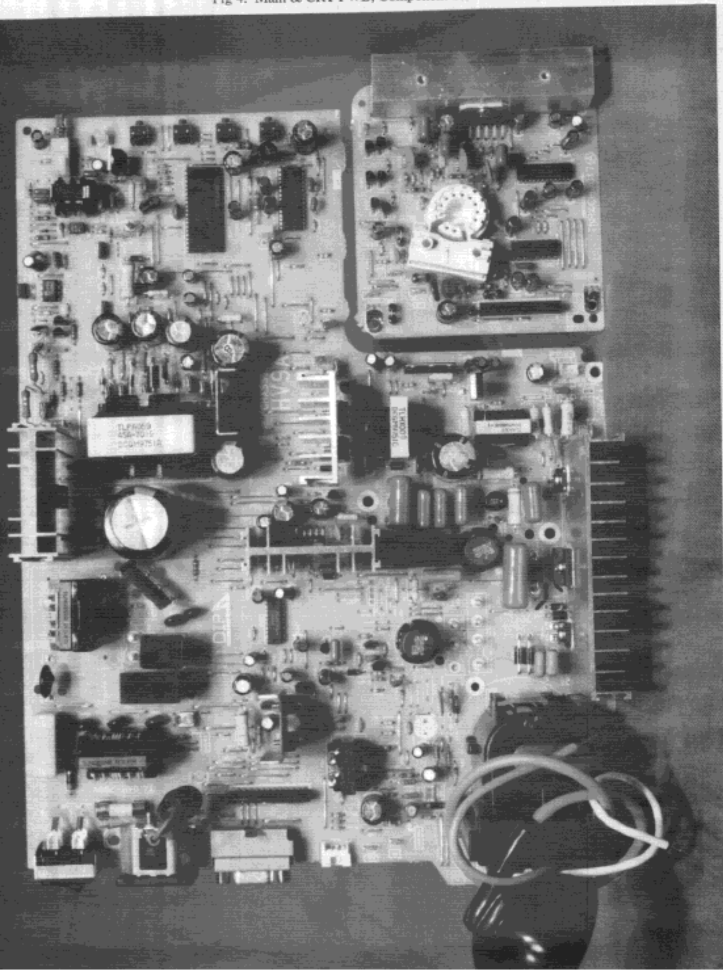
Fig 4. Main & CRT PWB, Component Side
