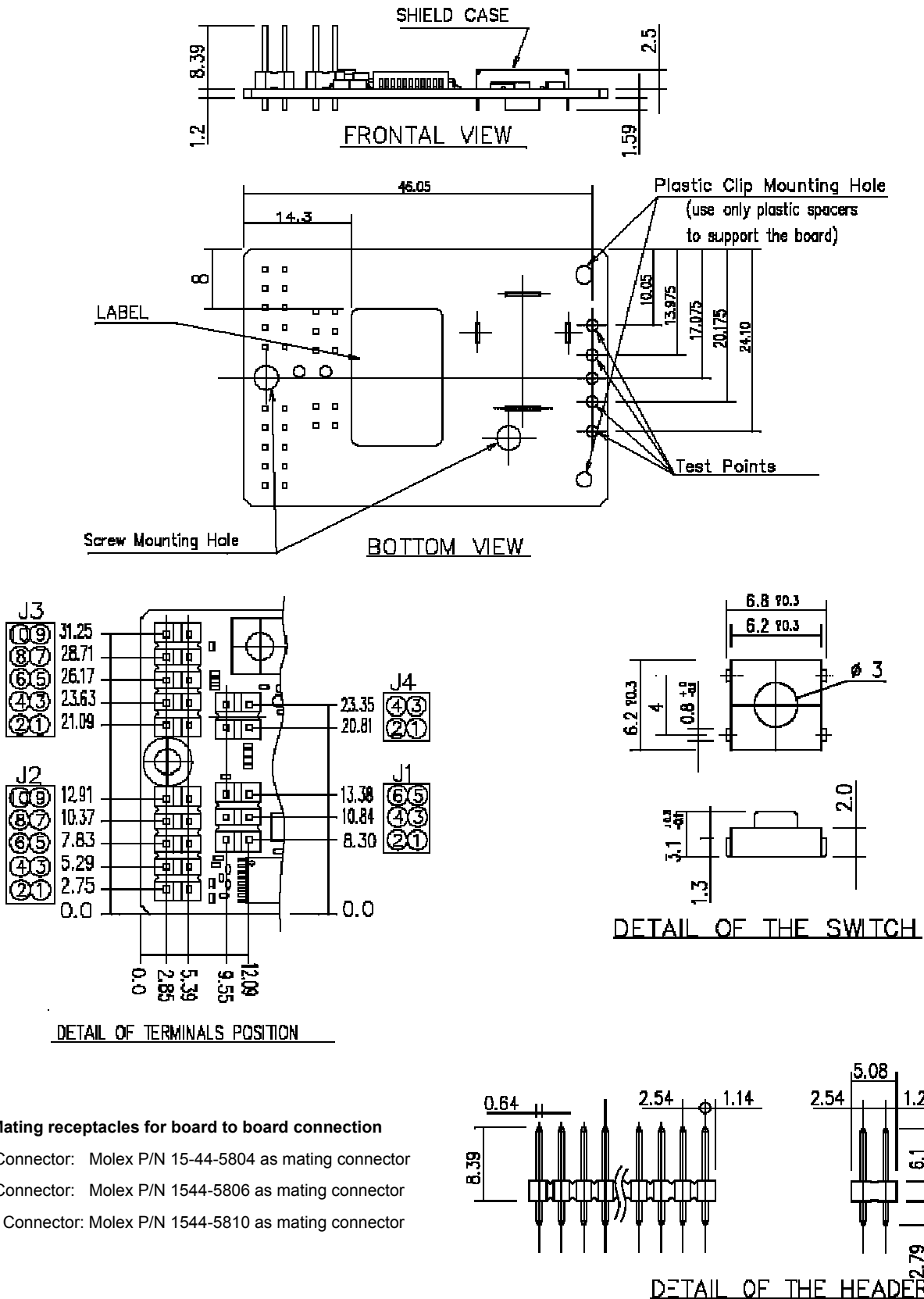
Figure 5: Mechanical drawing
