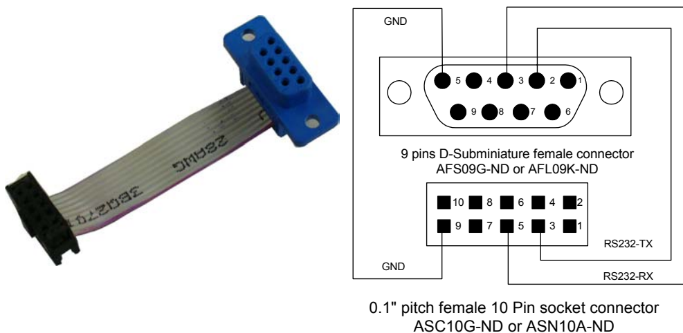
Figure 4: Serial interface cable from PAN802154 to Computer RS232
