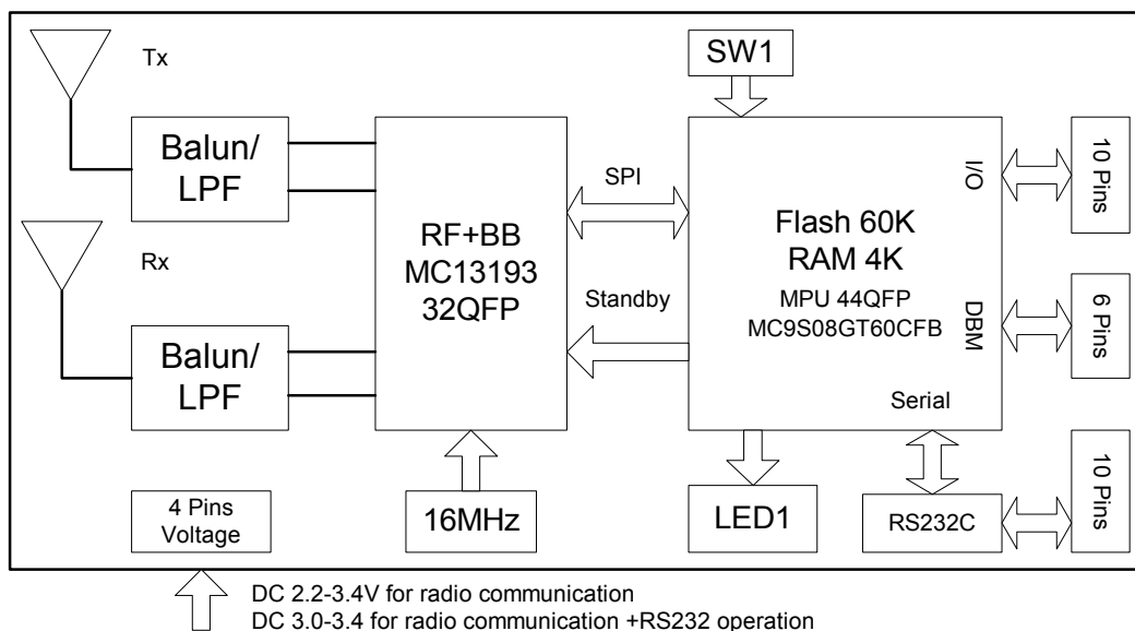
Figure 3: Block Diagram
