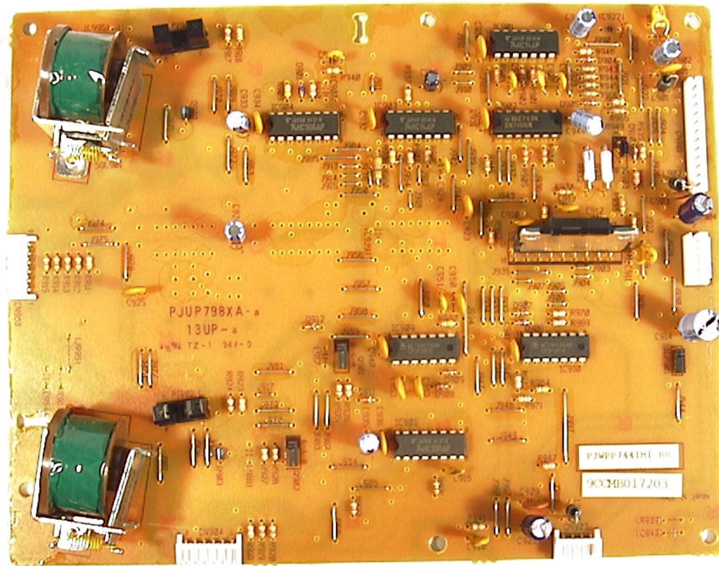
Photo.22 Top view of Second Cassette Feeder Board
