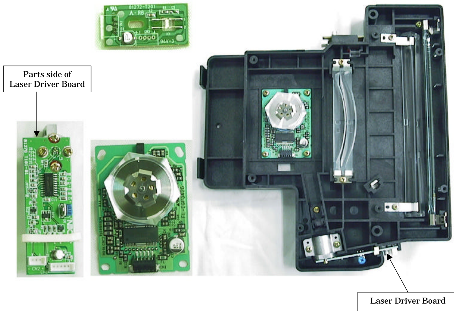
Photo.20 Top inside view of LSU and Circuit Board on LSU
