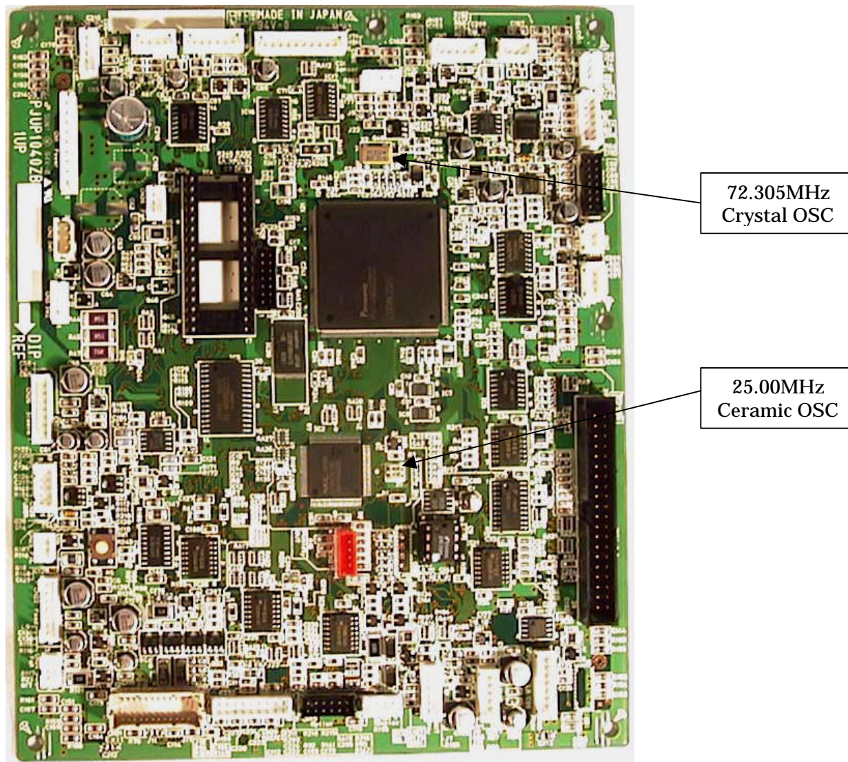
Photo.15 Top view of Printer Engine Control Board
