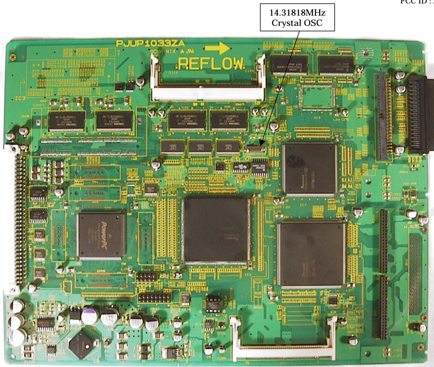
Photo.7 Top view of Main Control Board
