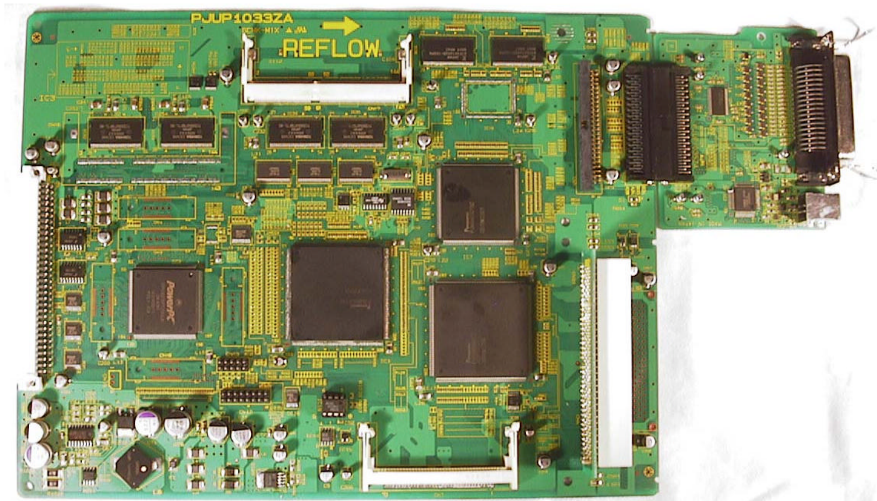
Photo.6 Top view of Main Control Board with P1284 & USB Interface Board and PCI Extension Board
