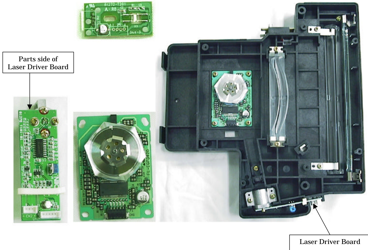
Photo.17 Top inside view of LSU and Circuit Board on LSU
