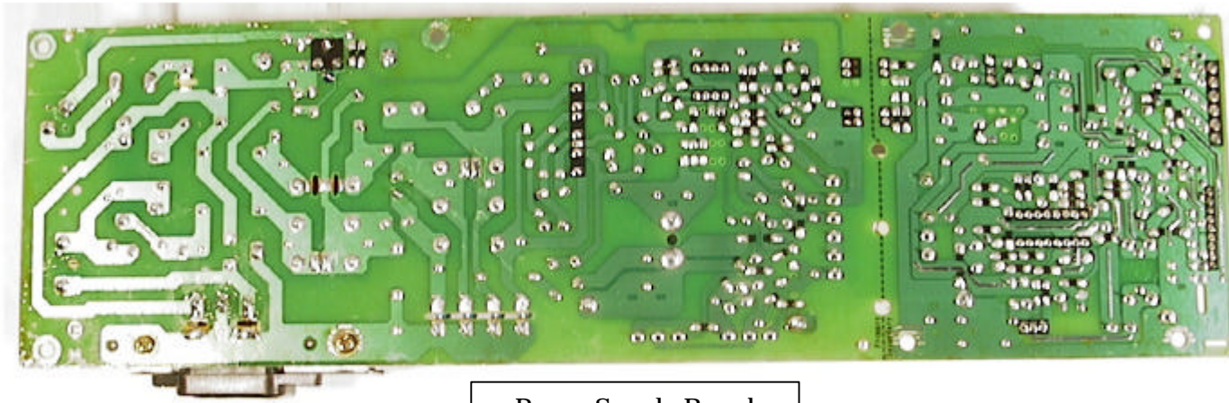
Power Supply Board
