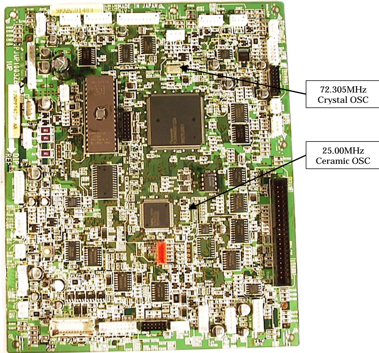
Photo.12 Top view of Printer Engine Control Board
