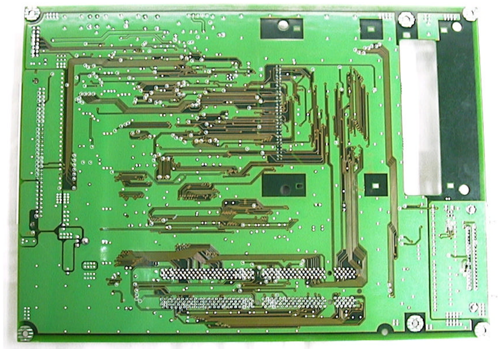
Photo.7 Bottom view of Main Control Board
