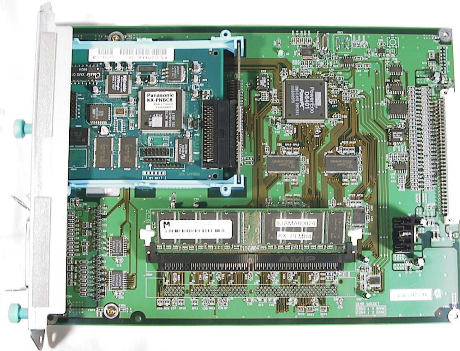
Photo.5 Top view of Main Control Board with Frame, option Network Card and expansion DIMM option added
