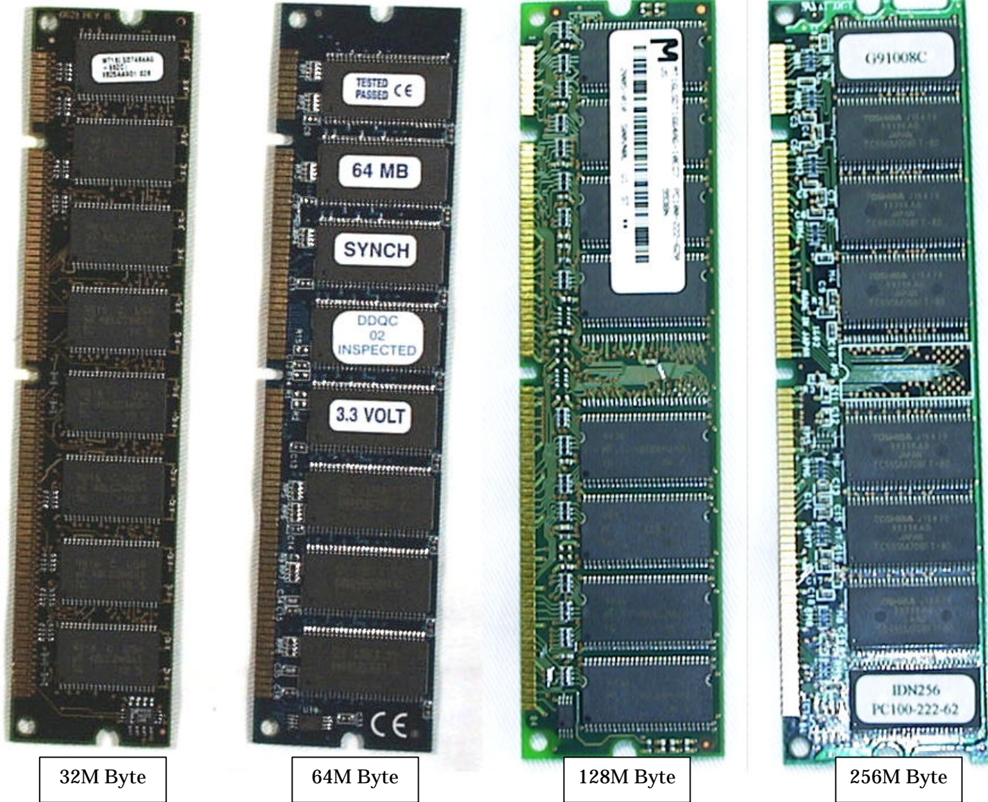
Photo.8 Top view of option DIMM Board
