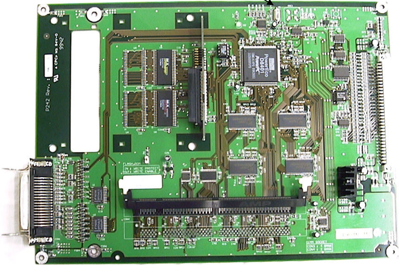
Photo.6 Top view of Main Control Board
