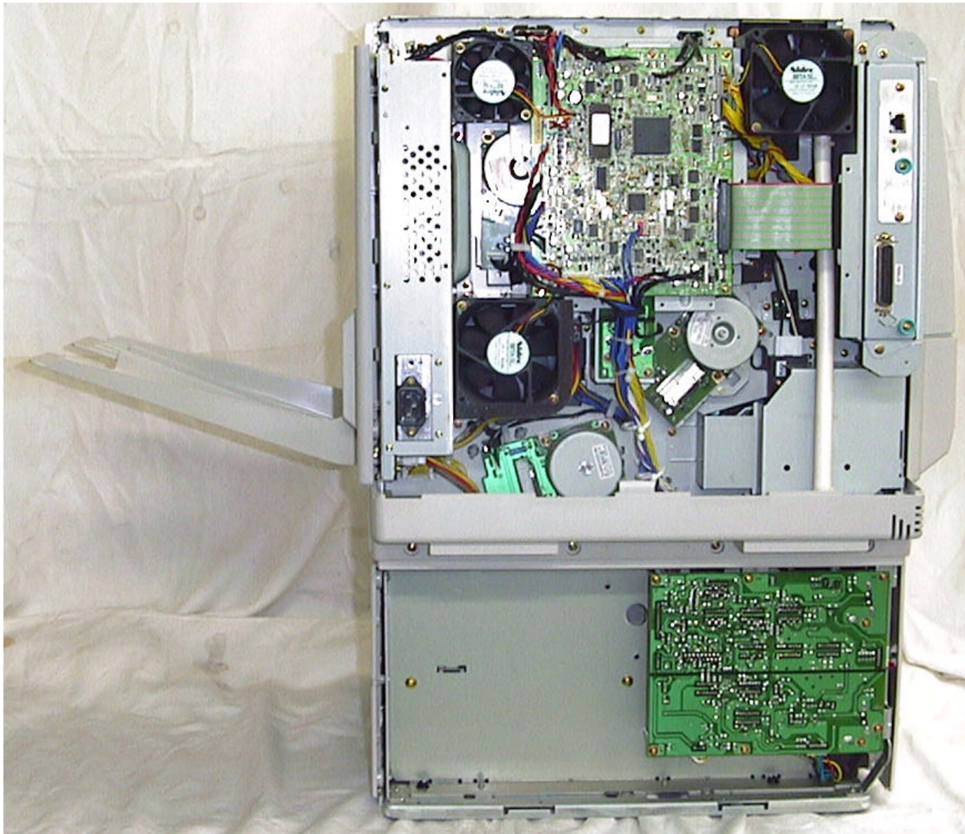
Photo.3 Rear inside view of the EUT with Rear Cabinet and Engine Board Cover removed
