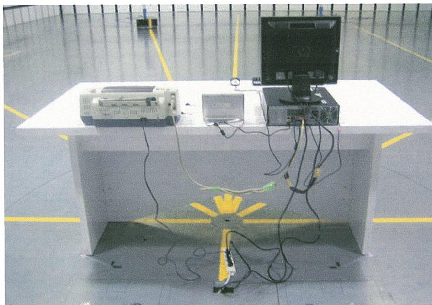
Test Configuration - Rear View
