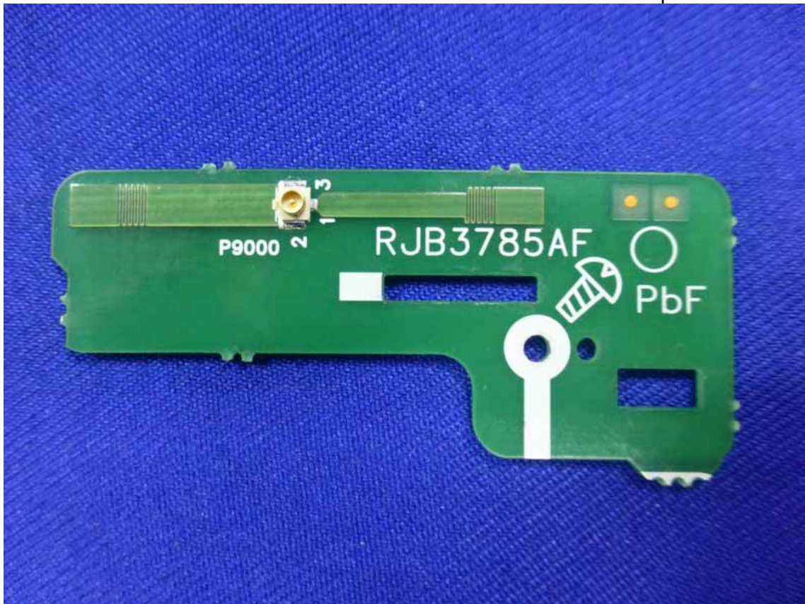
Figure 26 Component side of the Board
