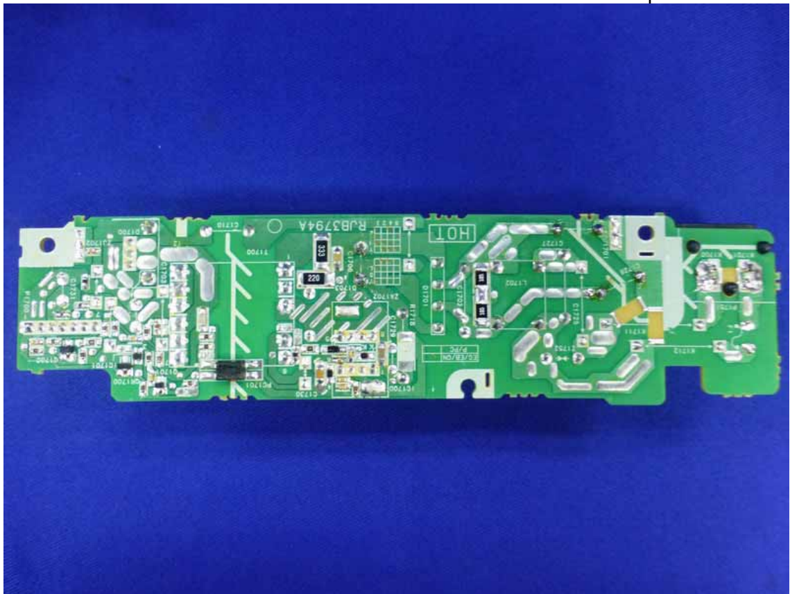
Figure 24 Component side of the Board
