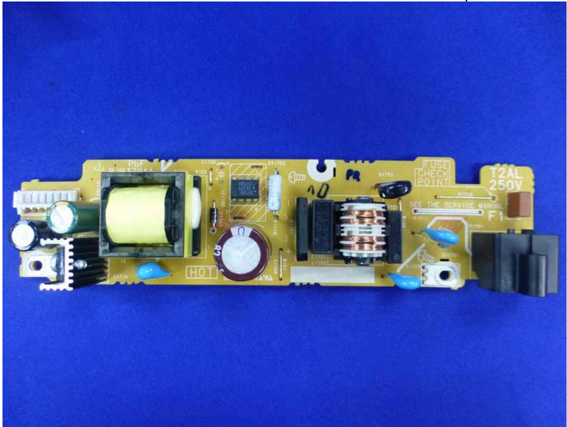
Figure 23 Component side of the Board
