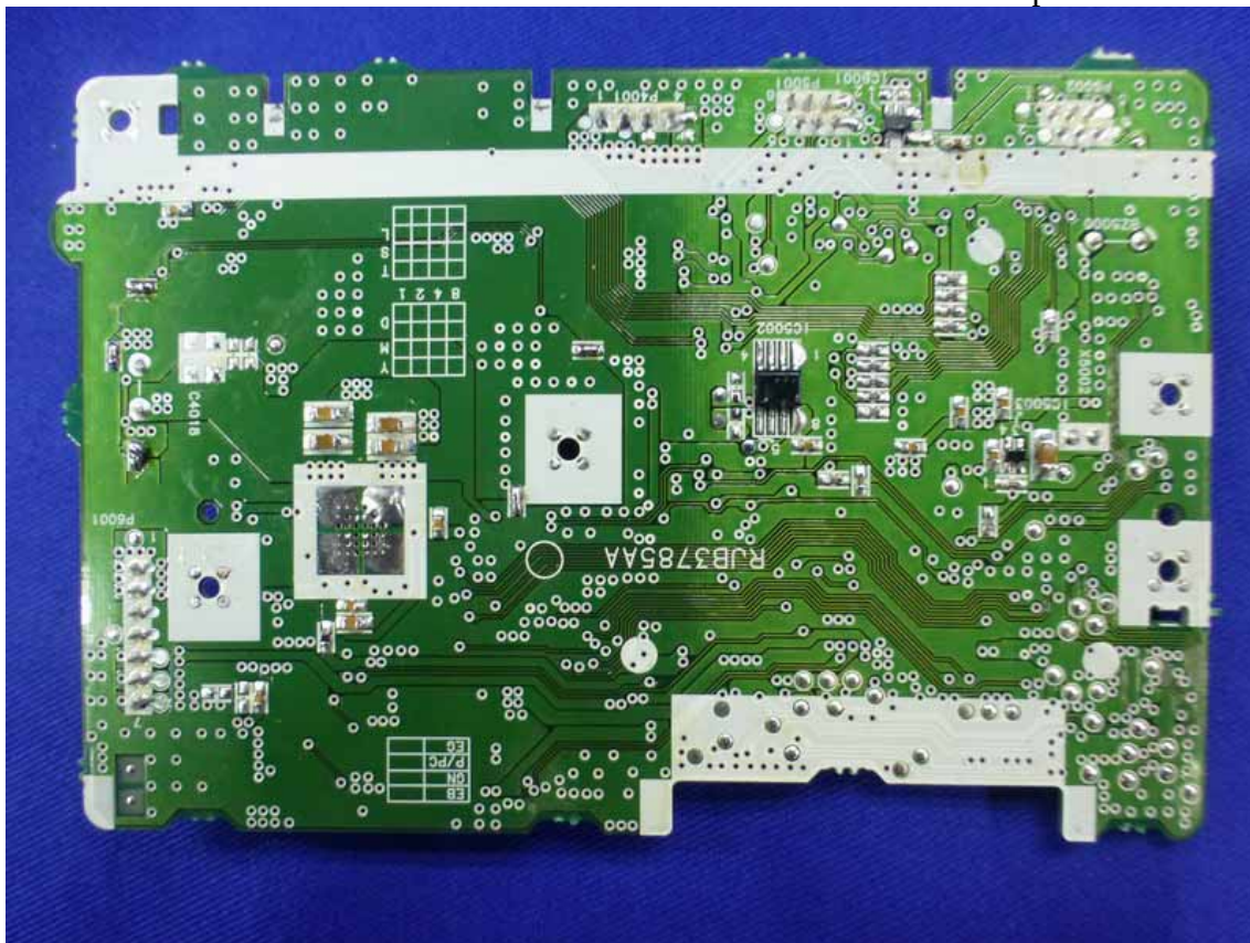
Figure 18 Component side of the Board
