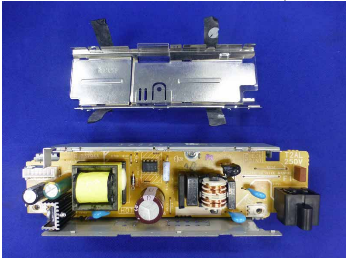
Figure 22 Component side of the Board
