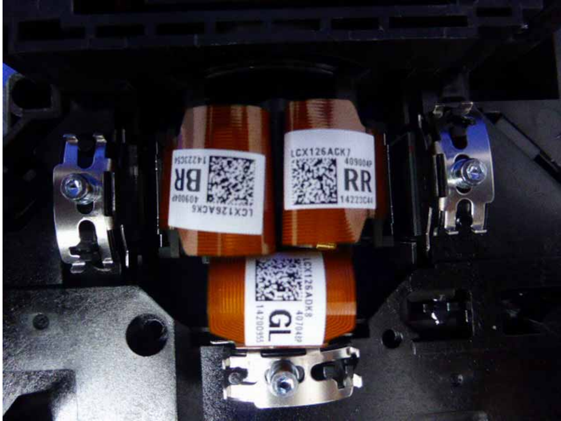
Figure 49 Inside of the EUT
