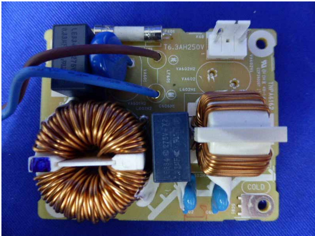
Figure 44 Inside of the EUT
