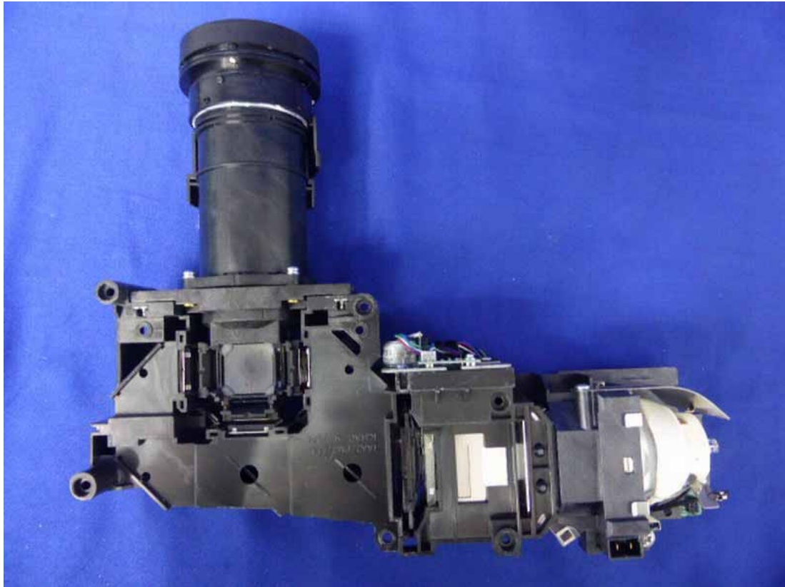
Figure 50 Inside of the EUT
