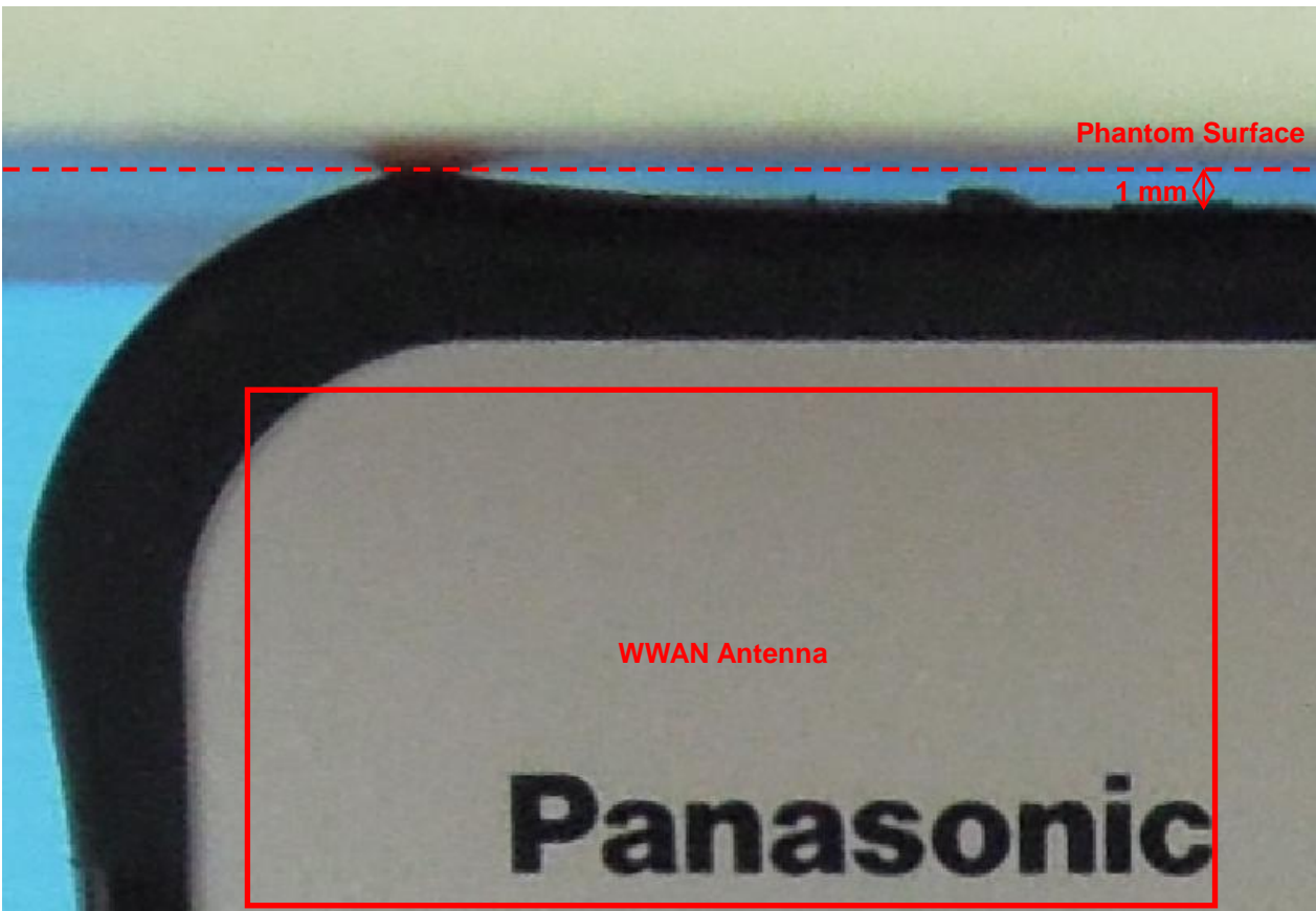
SAR Test Position : Secondary Portrait with 0 mm Gap
