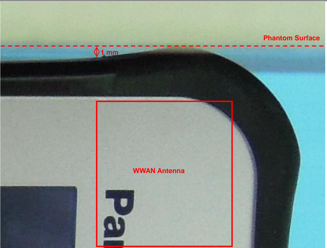
SAR Test Position : Primary Landscape with 0 mm Gap
