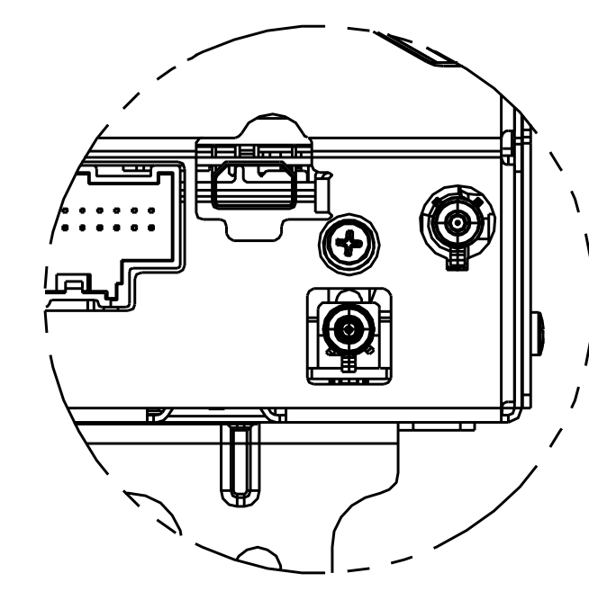
DETAIL C CDT+XM REAR VIEW
