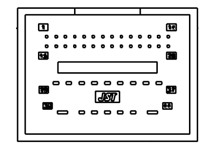
MAIN CONNECTOR J1 (JST 44 WAY) PIN OUT DIAGRAM
