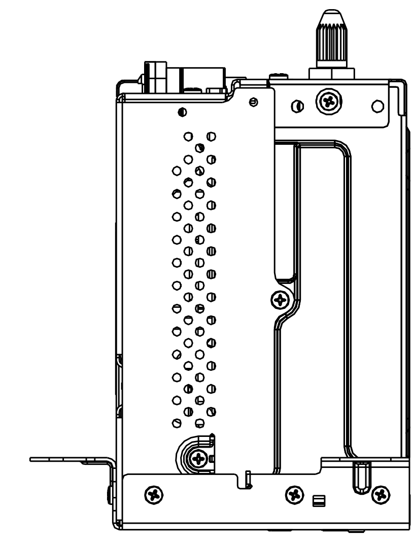
CDT RIGHT SIDE VIEW
