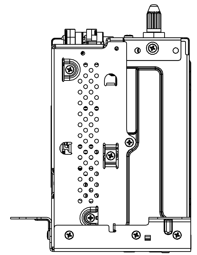
CDT+XM RIGHT SIDE VIEW
