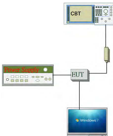
Fig. 2-1 Radiated Emission & Conducted Emission (Antenna Port) Configuration
