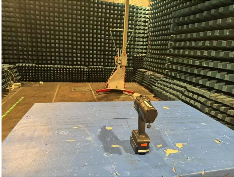
Test setup photo for radiated emission test (30MHz-1GHz)
