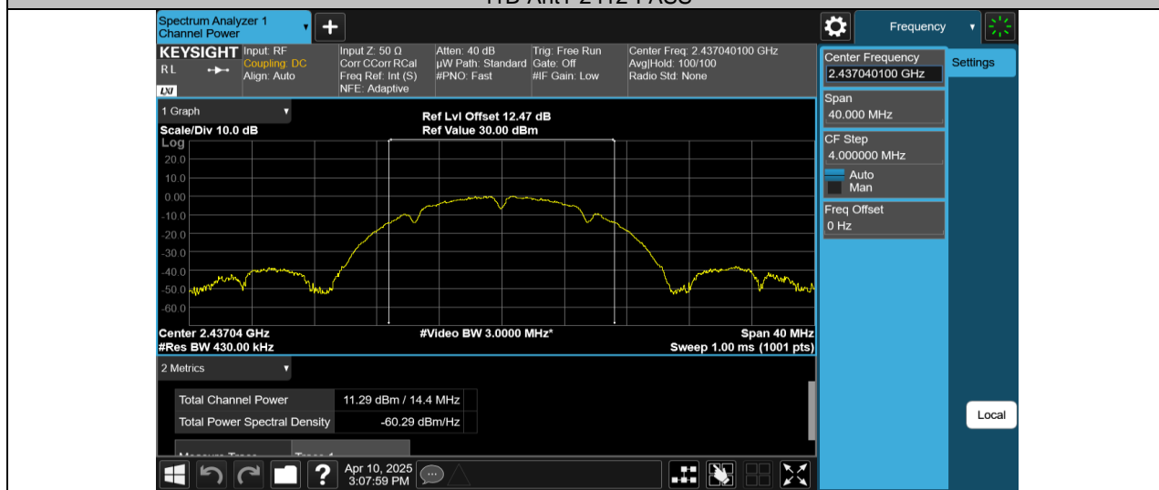
11B-Ant1-2437-PASS
