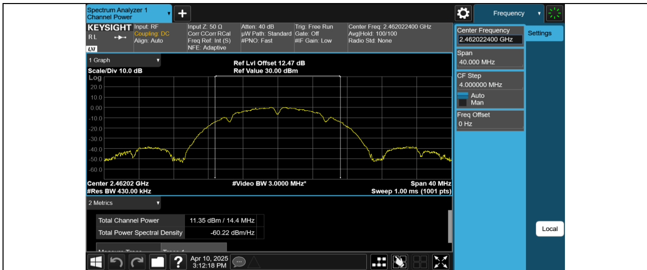
11B-Ant1-2462-PASS
