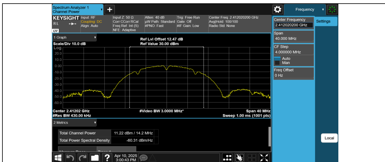
11B-Ant1-2412-PASS
