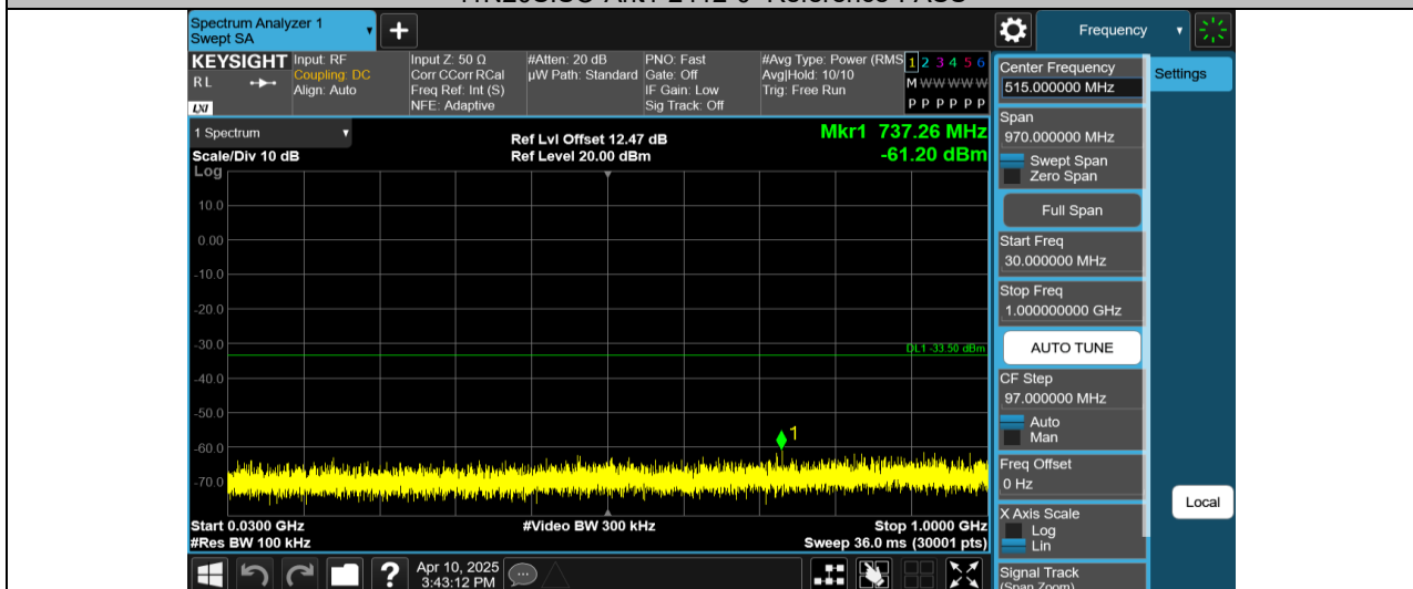
11N20SISO-Ant1-2412-30~1000-PASS
