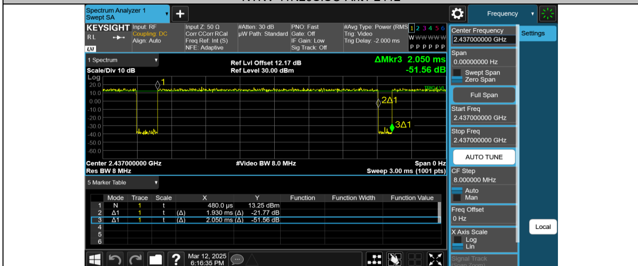
NTNV-11N20SISO-Ant1-2437
