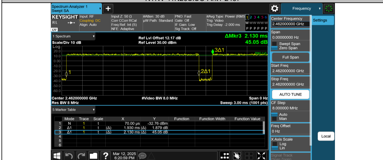
NTNV-11N20SISO-Ant1-2462
