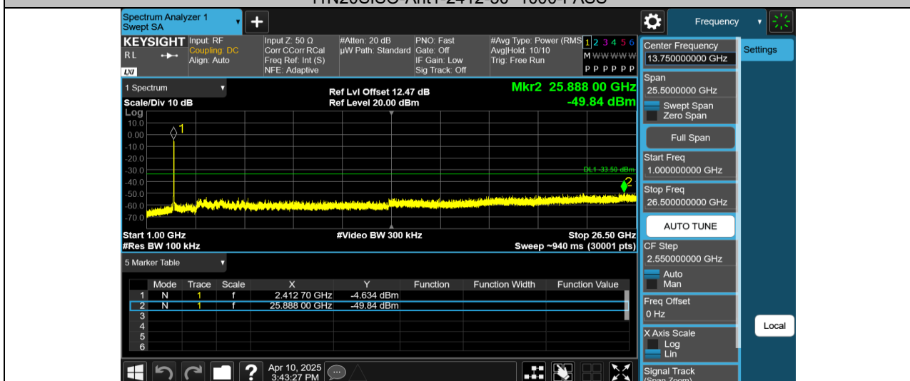
11N20SISO-Ant1-2412-1000~26500-PASS
