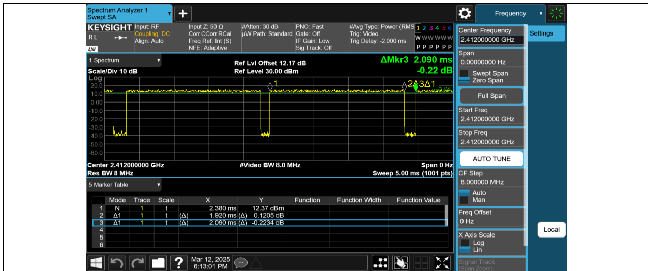
NTNV-11N20SISO-Ant1-2412
