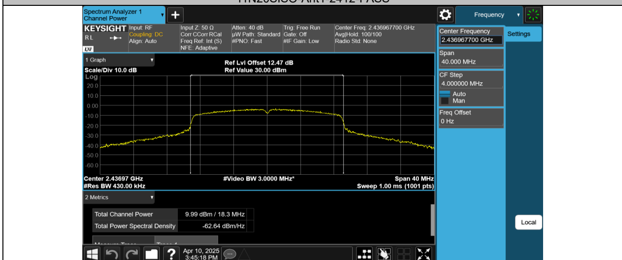
11N20SISO-Ant1-2437-PASS
