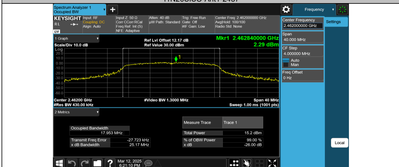
11N20SISO-Ant1-2462
