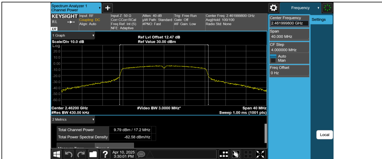
11G-Ant1-2462-PASS
