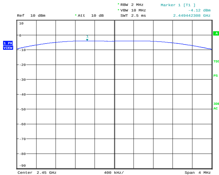
Figure 4: Conducted Output Power, Mode B (2450MHz), Worst Case Input Voltage (DC 3.7V)
