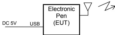
Figure 1: Block Diagram 1
