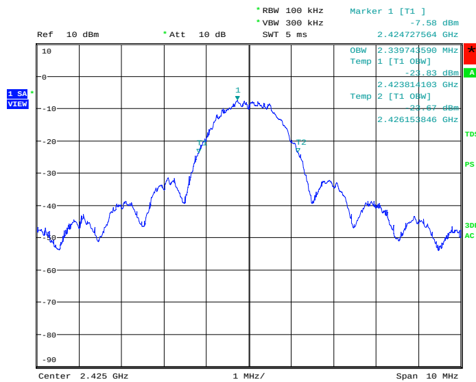
Figure 9: 99% Bandwidth, Mode A (2425MHz)
