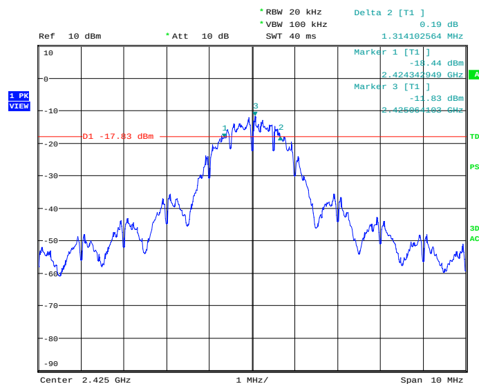
Figure 6: 6dB Bandwidth, Mode A (2425MHz)
