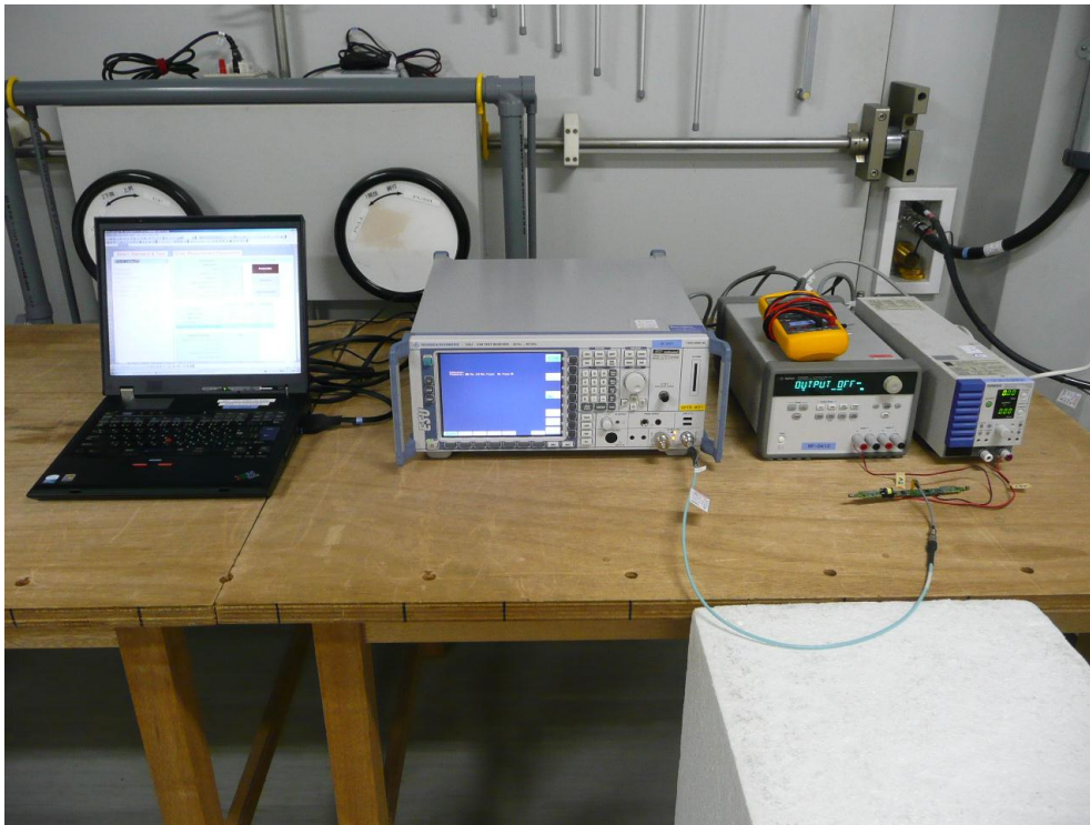
Photograph 2: Set-up for AC Power Line Conducted Emission of Transmitter
