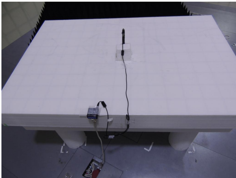
Photograph 3: Set-up for Radiated Emission of Transmitter
