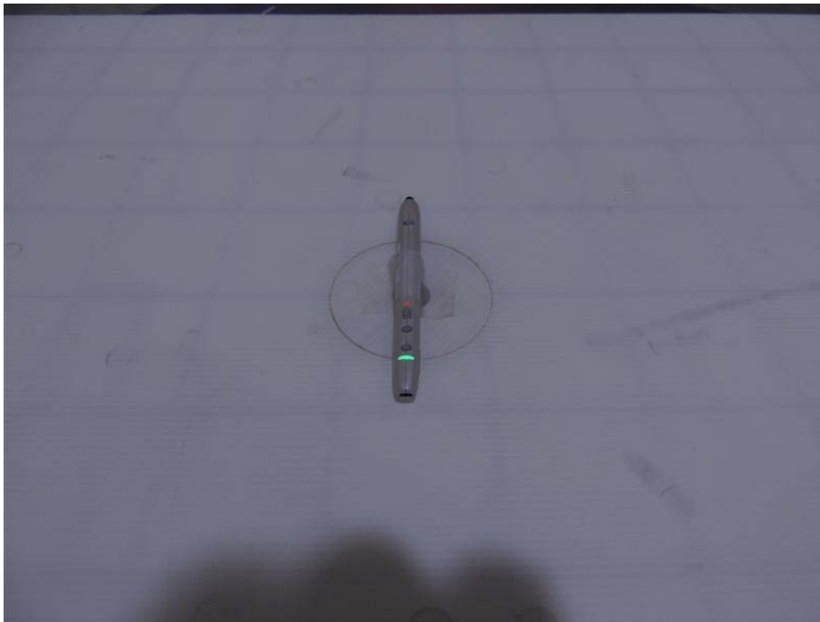
Photograph 3: Set-up for Radiated Emission, EUT Configuration X-Axis
