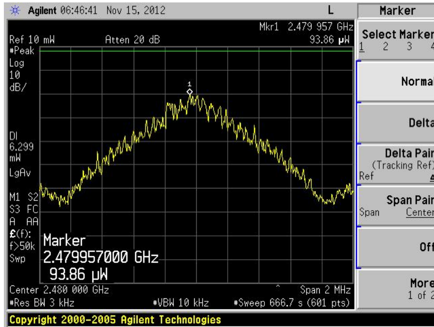
Plot 45 – Channel 78 (upper ch)
