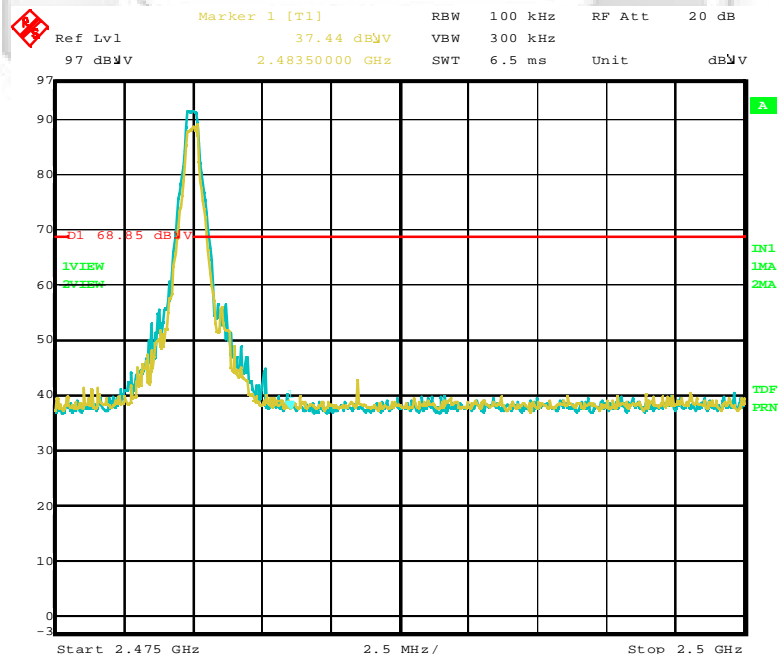
Plot 38 – Upper Band Edge at 2.4835GHz
