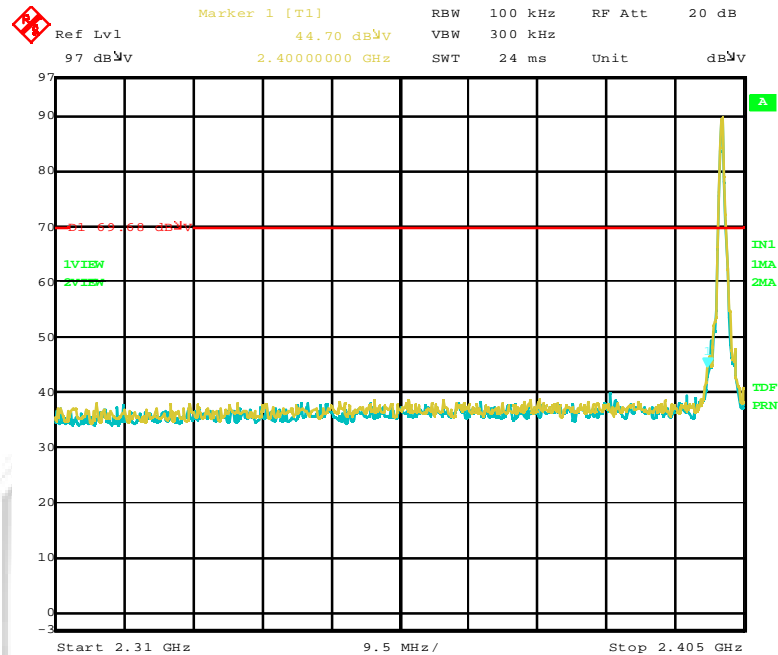
Plot 37 – Lower Band Edge at 2.400GHz
