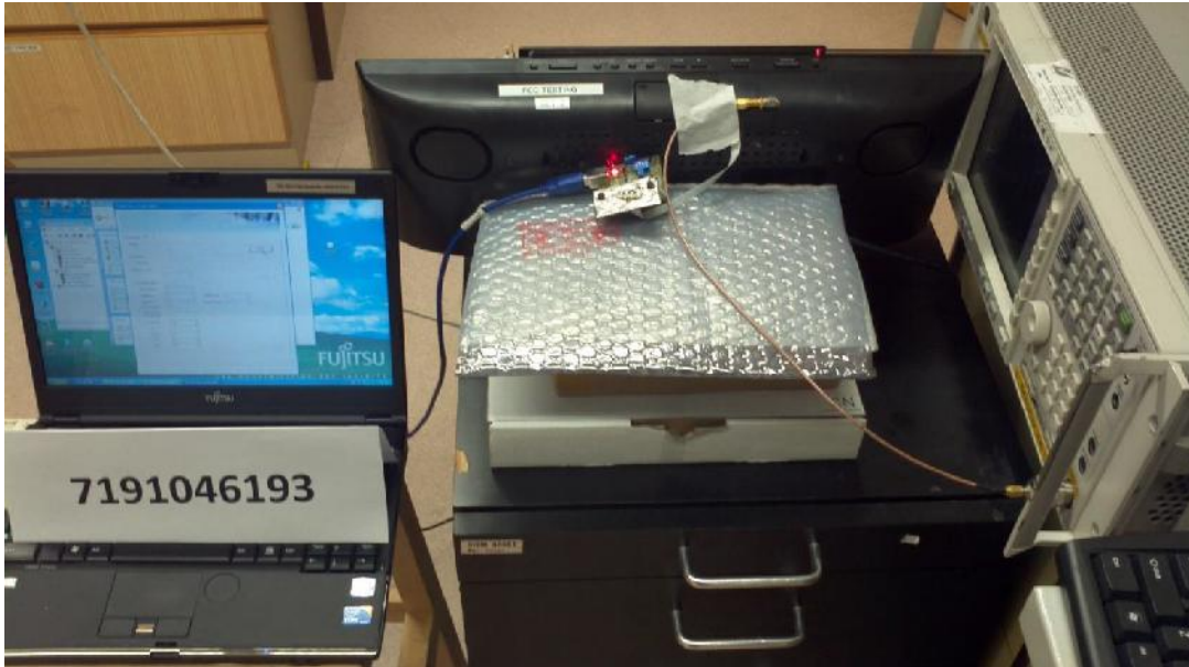
Carrier Frequency Separation Test Setup
