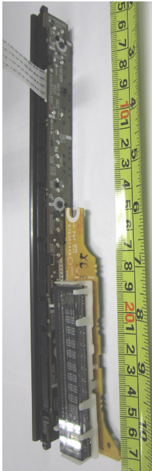
Front Panel LCD Board PCB Component Side
