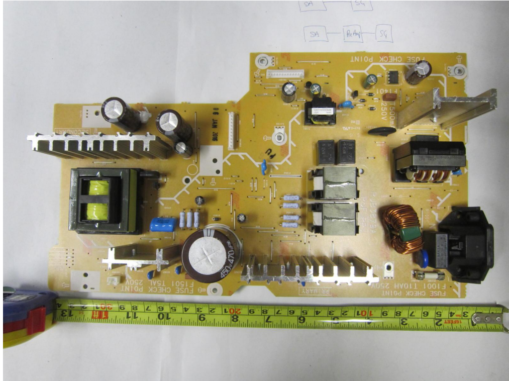
Power Supply Board PCB Component Side
