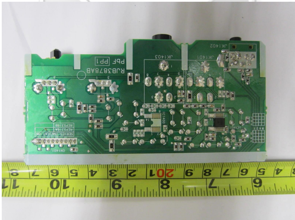
Sub-Board 1 PCB Trace Side
