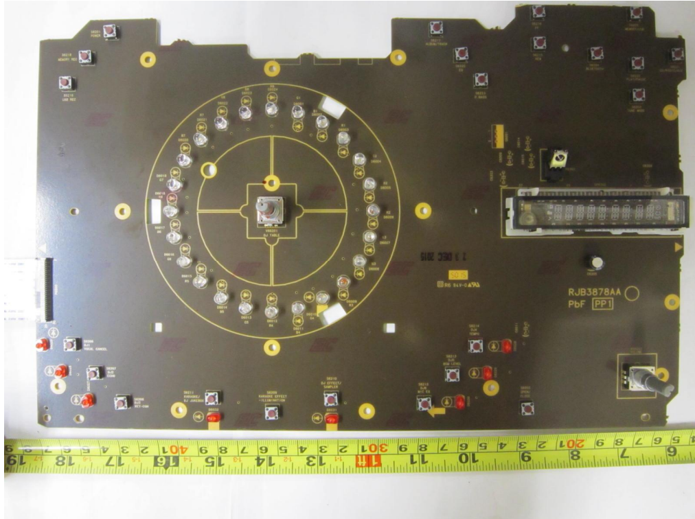
LCD Display Board PCB Component Side
