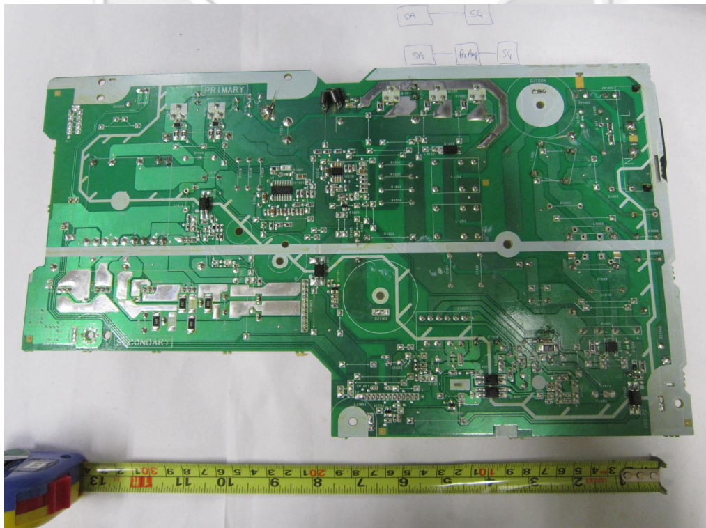
Power Supply Board PCB Trace Side
