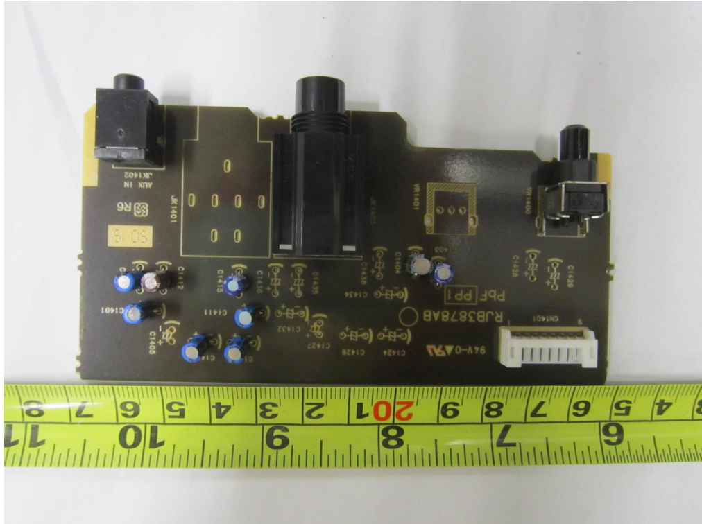
Sub-Board 1 PCB Component Side
