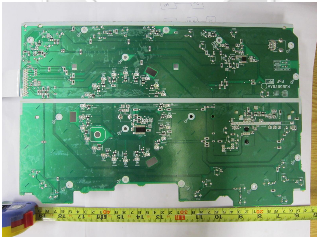
LCD Display Board PCB Trace Side
