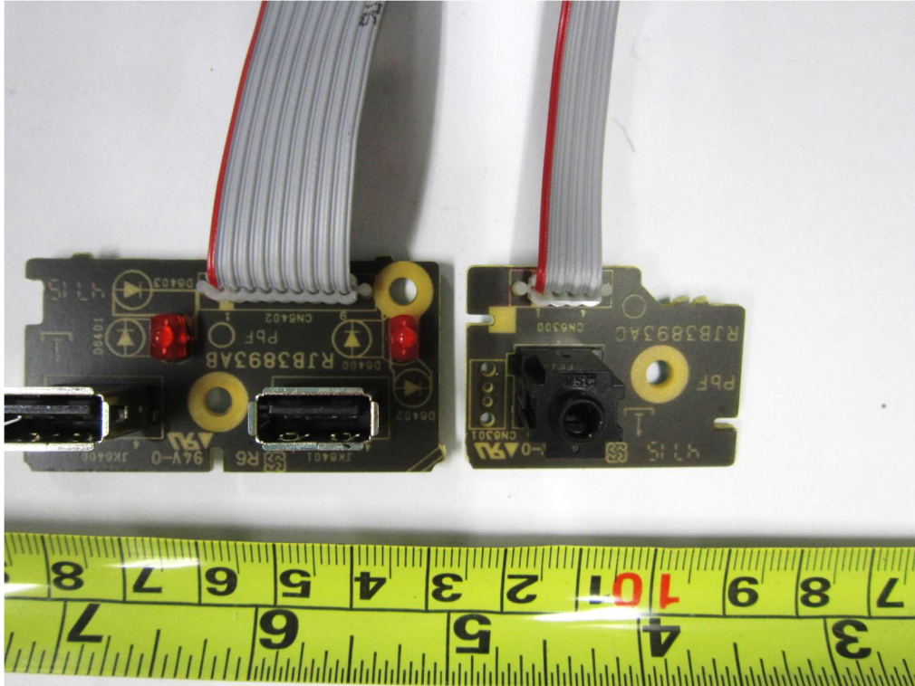
Sub-Board 2 PCB Component Side
