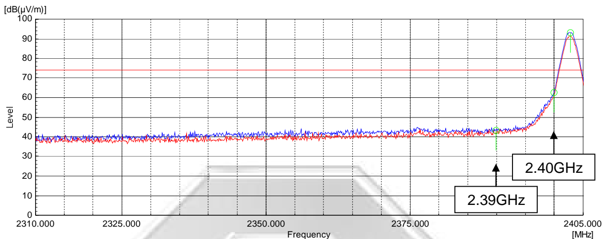
Plot 65 – Peak Plot at Lower Band Edge at 2.4000GHz
