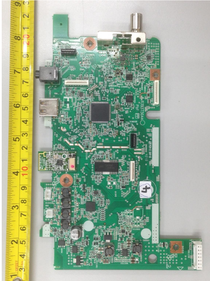
Main-Board PCB Component Side
