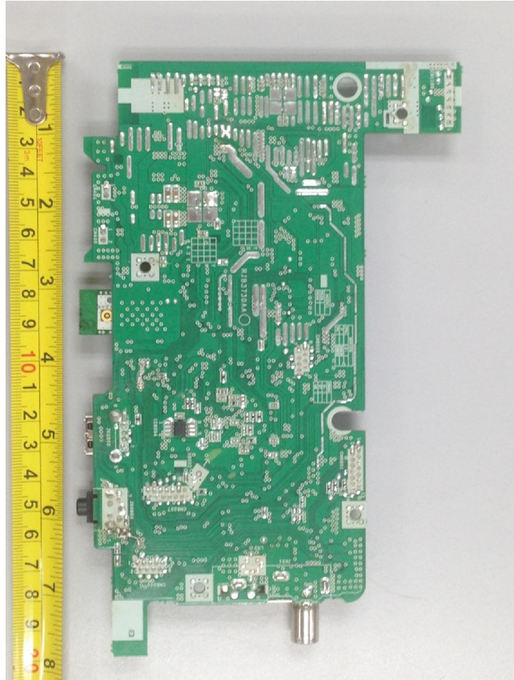
Main-Board PCB Trace Side
