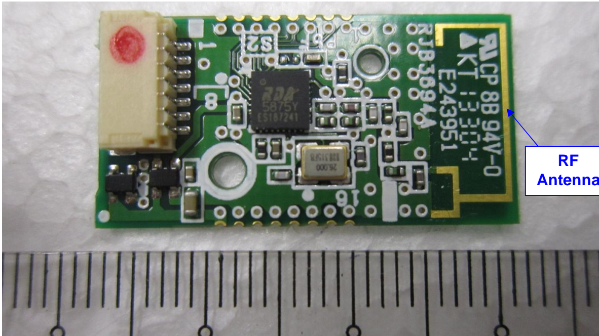
RF Module Circuit Component Side
