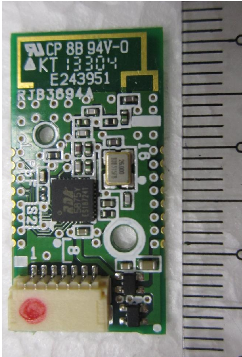
RF Module Circuit Component Side
