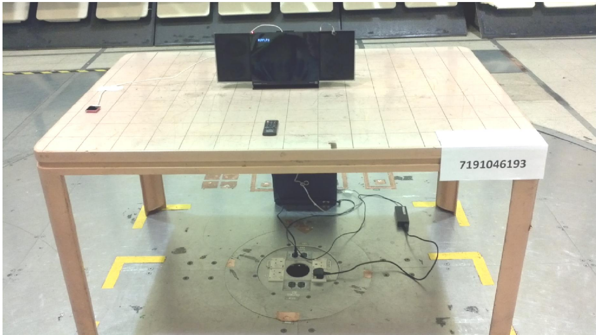
Radiated Emissions Test Setup (Front View)
