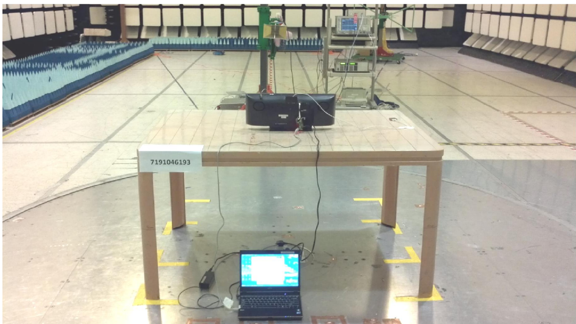
Radiated Emissions Test Setup (Rear View)
