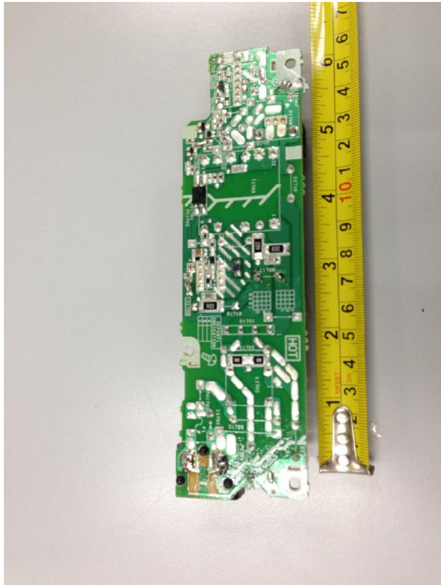
Power Supply Board PCB Trace Side
