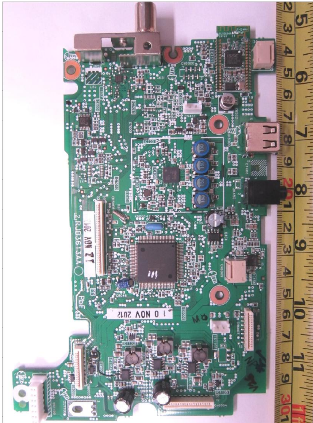
Main-Board PCB Component Side
