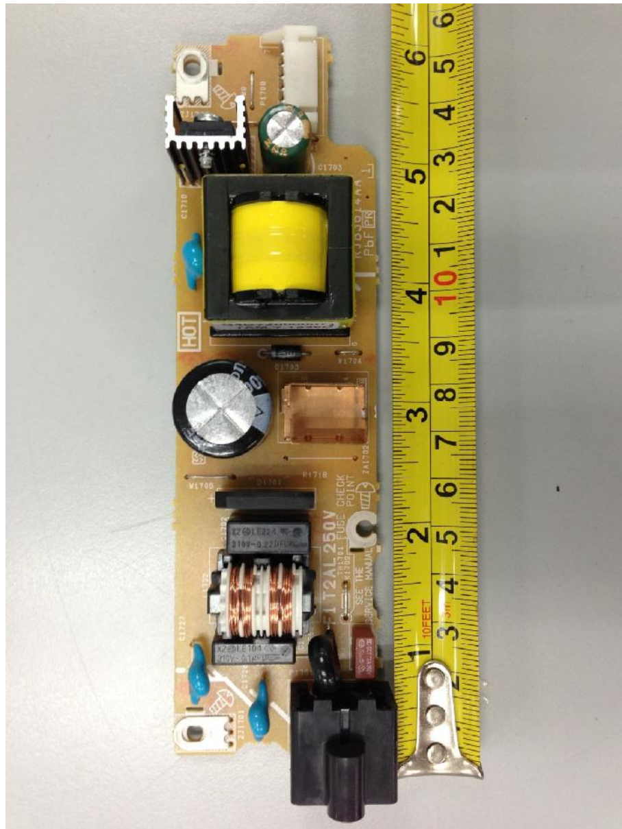
Power Supply Board PCB Component Side
