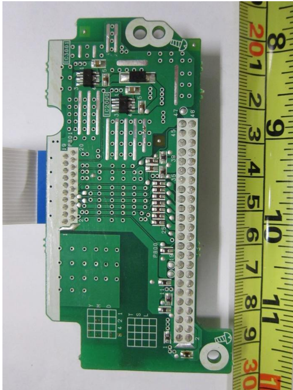
Bridge Board PCB Trace Side
