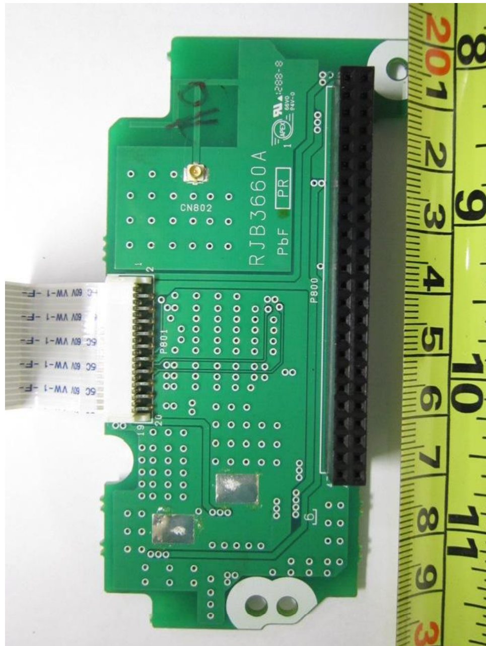
Bridge Board PCB Component Side
