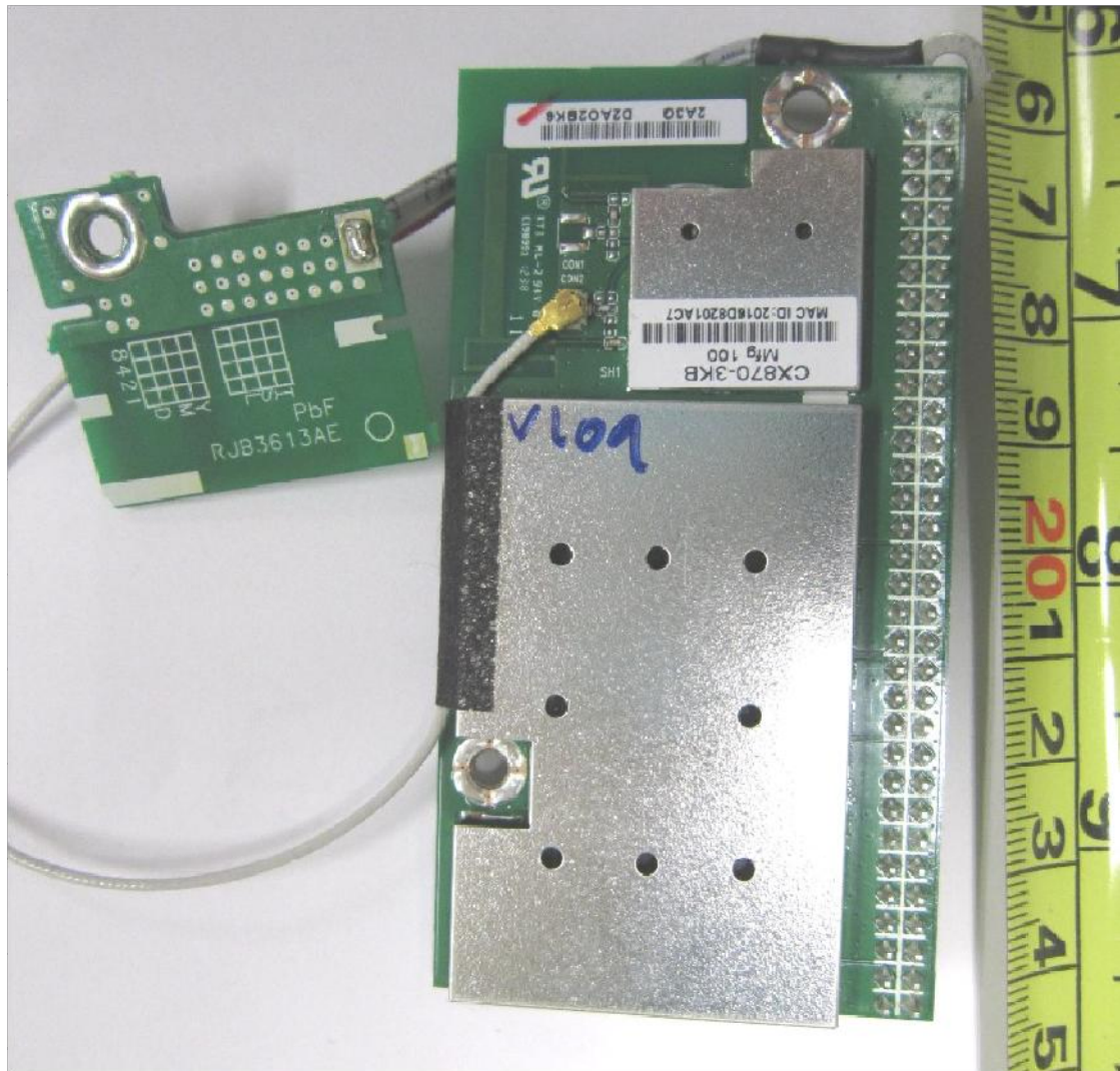
AirPlay Board & External Antennal Board
