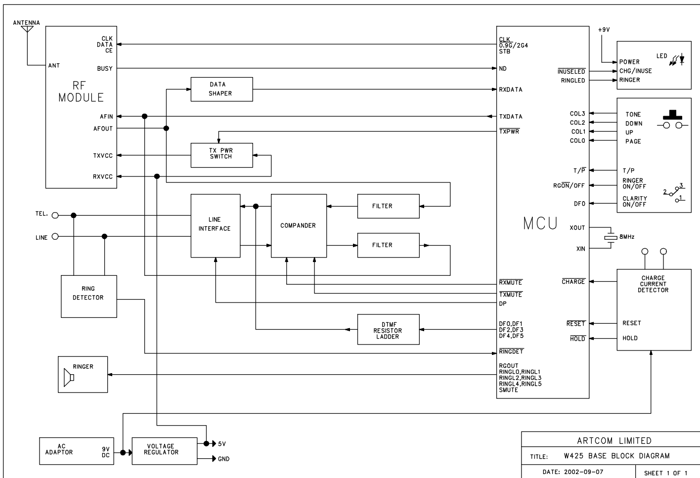
W425 Base Unit Block Diagram
