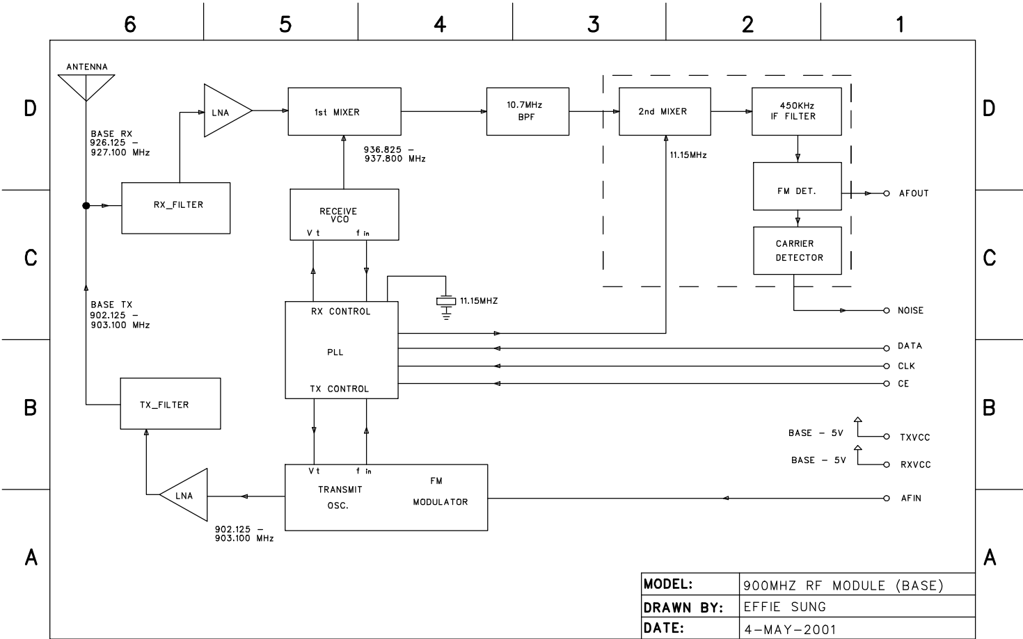
RF Module (Base) Block Diagram
