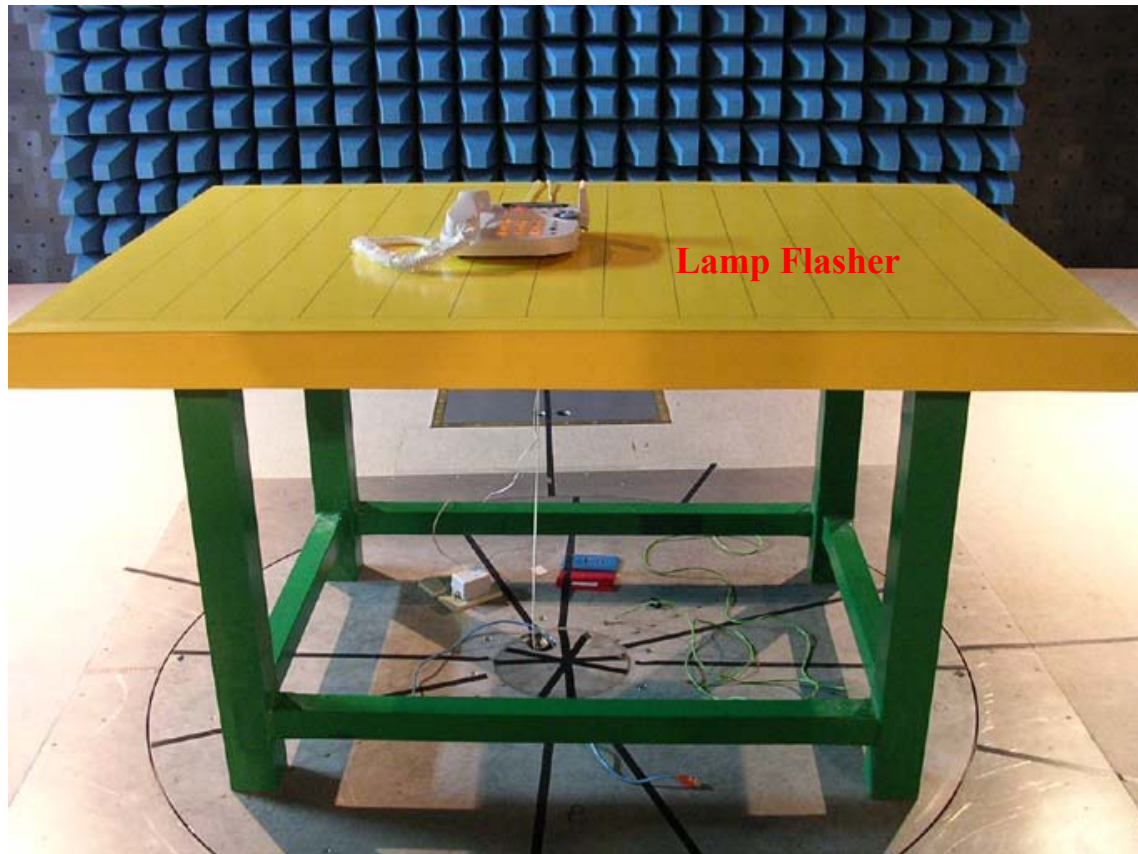
Photo 1: Tx Radiated Emission Set-up Photo
