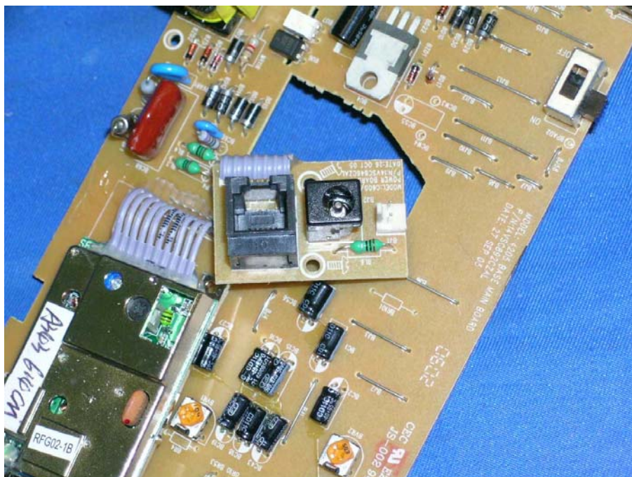
Base Unit Telephone and AC Jack front side
