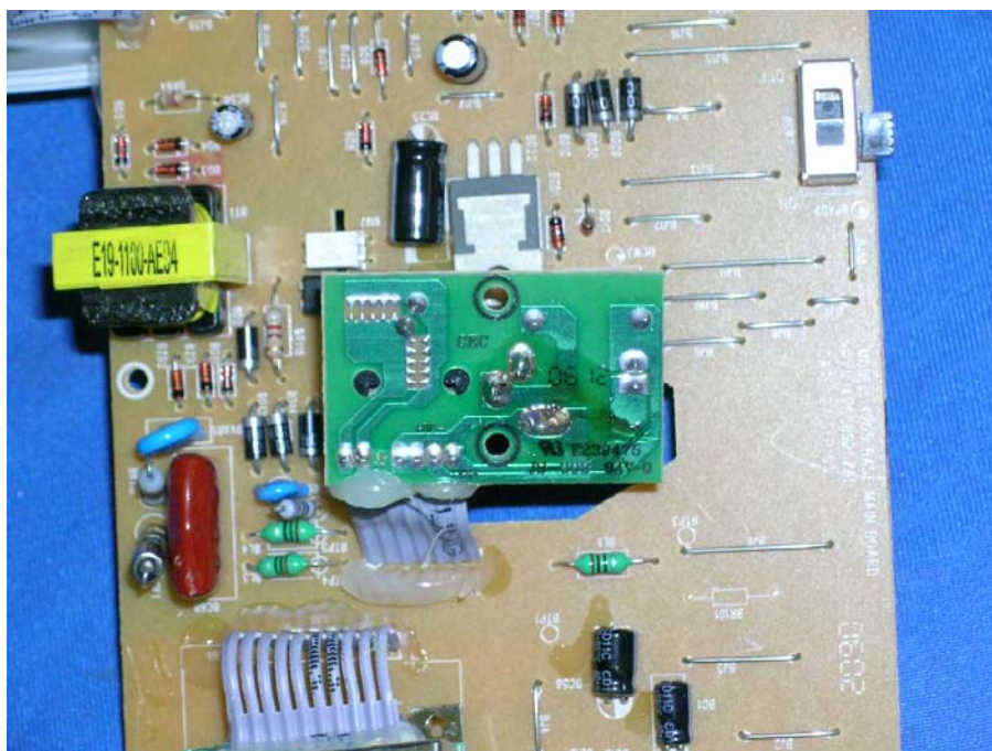
Base Unit Telephone and AC Jack rear side
