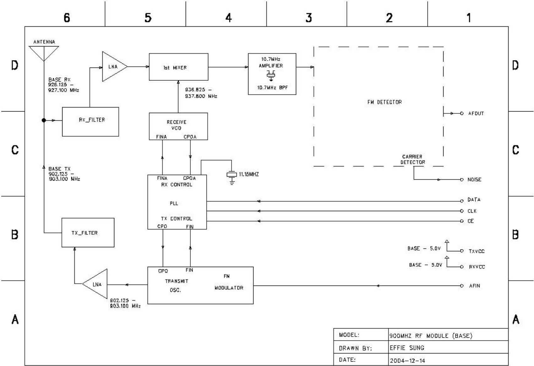
RF Module (Base) Block Diagram
