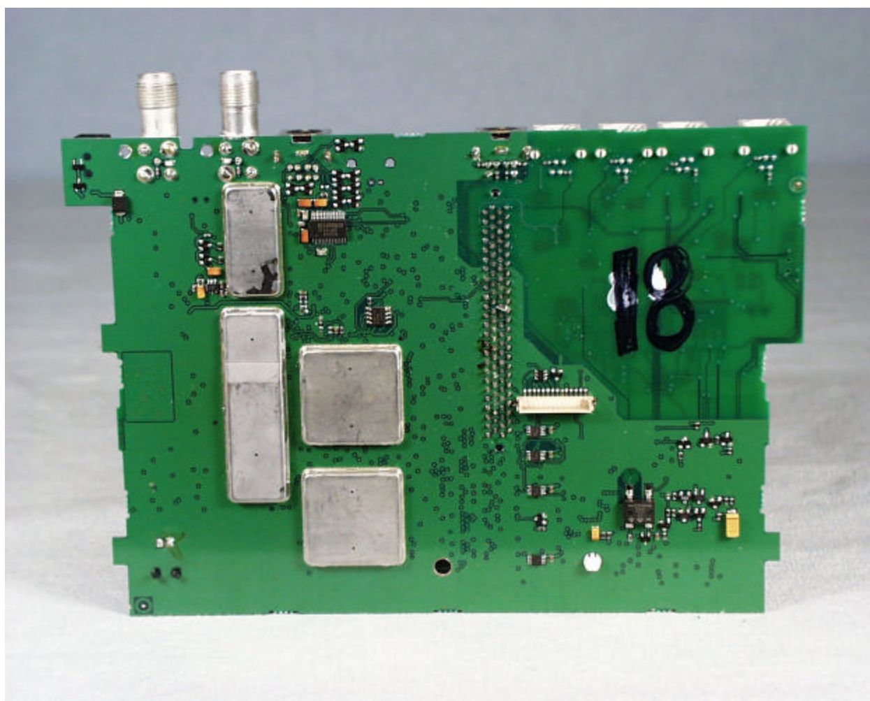
Solder side of RF Board
