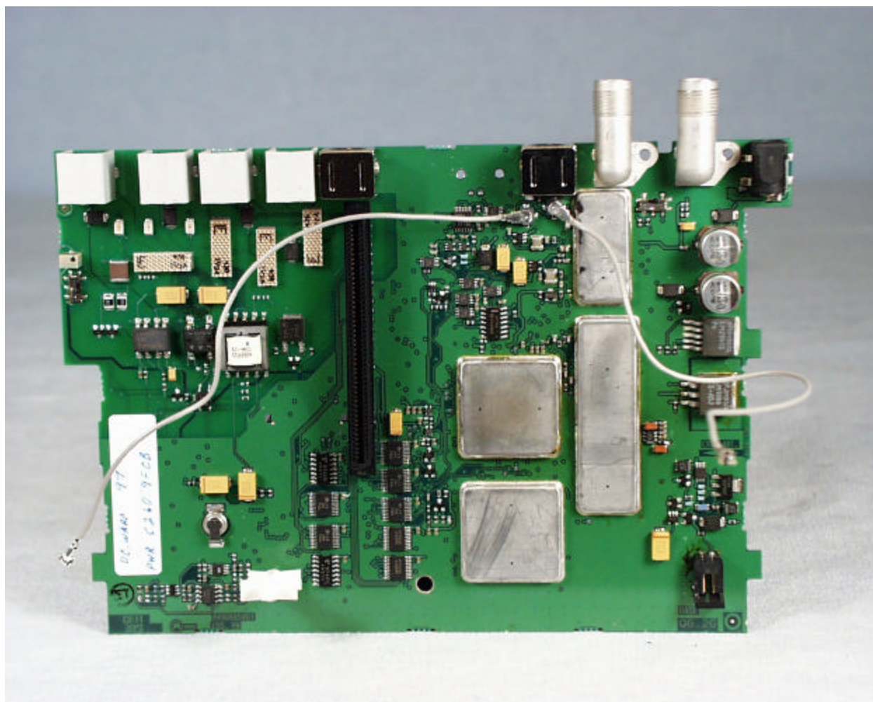
Component side of RF Board
