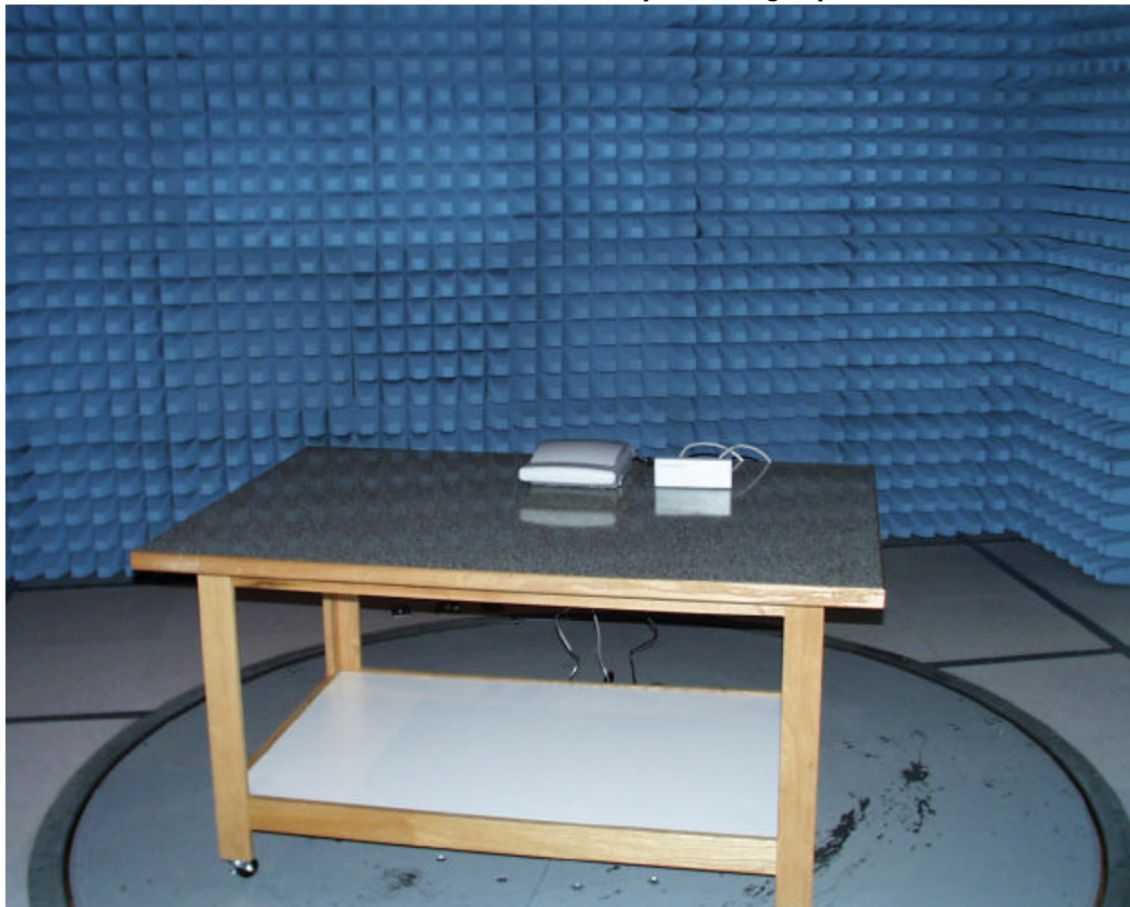
Front View of Worst Case Radiated and Line Conducted Emissions Test Set-up
