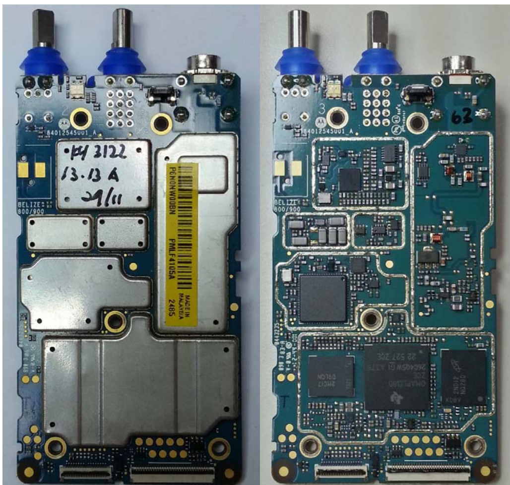
RF board with and without Shields (Top)
