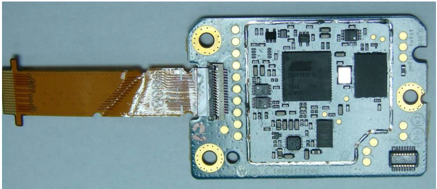
GOB board without shield (Bottom)
