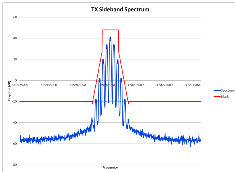
E1-5.41 Occupied Bandwidth, Analog, 12.5 kHz Channels, 469.9875 MHz PL
