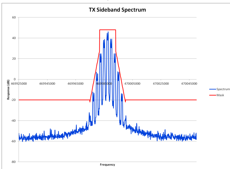
E1-5.42 Occupied Bandwidth, Analog, 12.5 kHz Channels, 469.9875 MHz DPL
