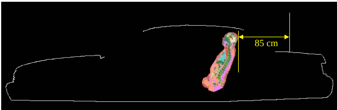
Figure 2: Passenger model exposed to a trunk-mount antenna: XFDTD geometry. The antenna is mounted at 85 cm from the passenger located in the center of the back seat.
