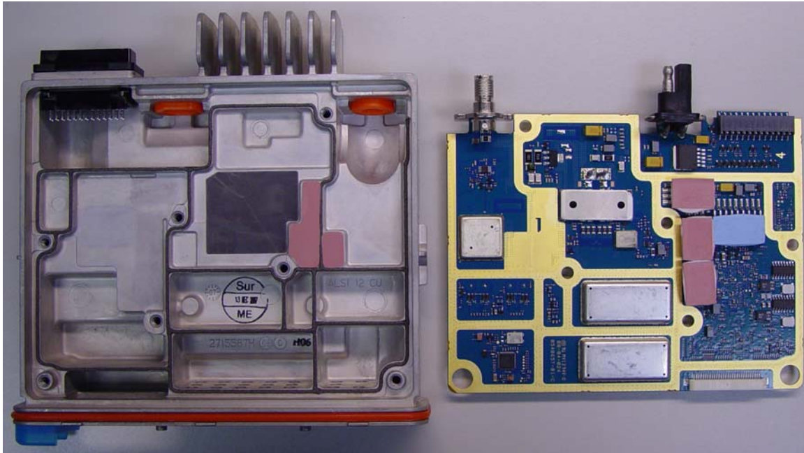
TOP VIEW OF NON-GPS MODEL WITH CIRCUIT BOARD REMOVED FROM CHASSIS (MATING SURFACES OF CIRCUIT BOARD AND CHASSIS ARE SHOWN)
