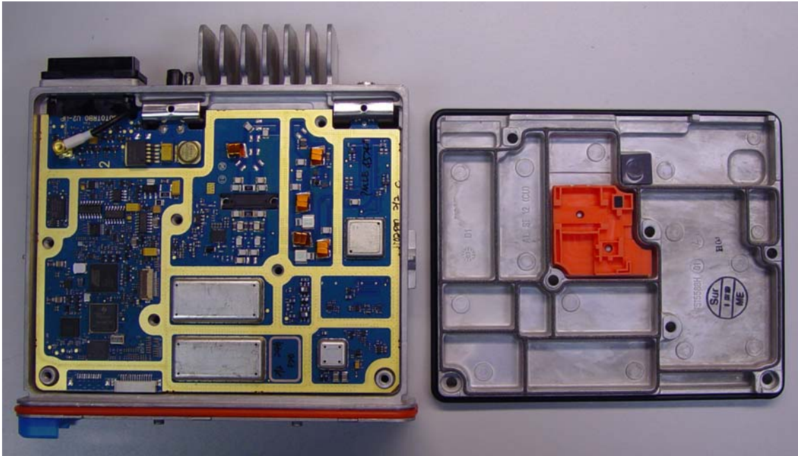
TOP VIEW OF GPS MODEL WITH CHASSIS TOP COVER REMOVED (MATING SURFACES OF TOP COVER AND CIRCUIT BOARD IN CHASSIS ARE SHOWN)
