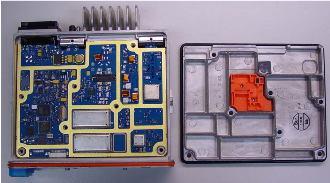
TOP VIEW OF NON-GPS MODEL WITH CHASSIS TOP COVER REMOVED (MATING SURFACES OF TOP COVER AND CIRCUIT BOARD IN CHASSIS ARE SHOWN)
