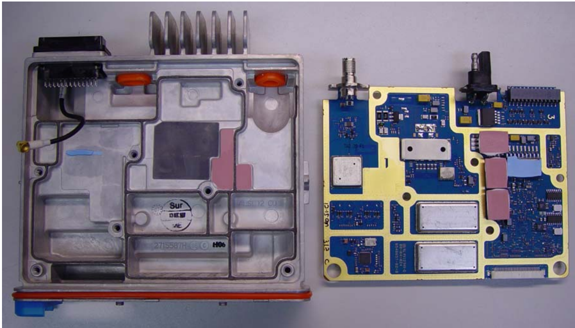
TOP VIEW OF GPS MODEL WITH CIRCUIT BOARD REMOVED FROM CHASSIS (MATING SURFACES OF CIRCUIT BOARD AND CHASSIS ARE SHOWN)
