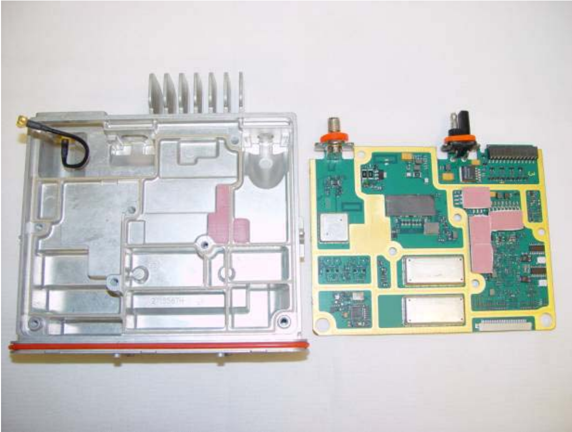
TOP VIEW OF GPS MODEL WITH CIRCUIT BOARD REMOVED FROM CHASSIS (MATING SURFACES OF CIRCUIT BOARD AND CHASSIS ARE SHOWN)
