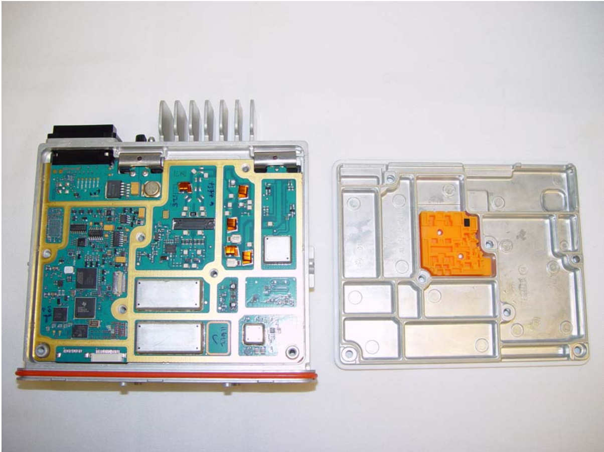
TOP VIEW OF NON-GPS MODEL WITH CHASSIS TOP COVER REMOVED (MATING SURFACES OF TOP COVER AND CIRCUIT BOARD IN CHASSIS ARE SHOWN)
