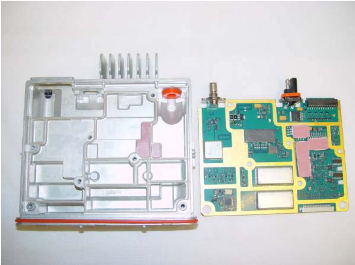
TOP VIEW OF NON-GPS MODEL WITH CIRCUIT BOARD REMOVED FROM CHASSIS (MATING SURFACES OF CIRCUIT BOARD AND CHASSIS ARE SHOWN)
