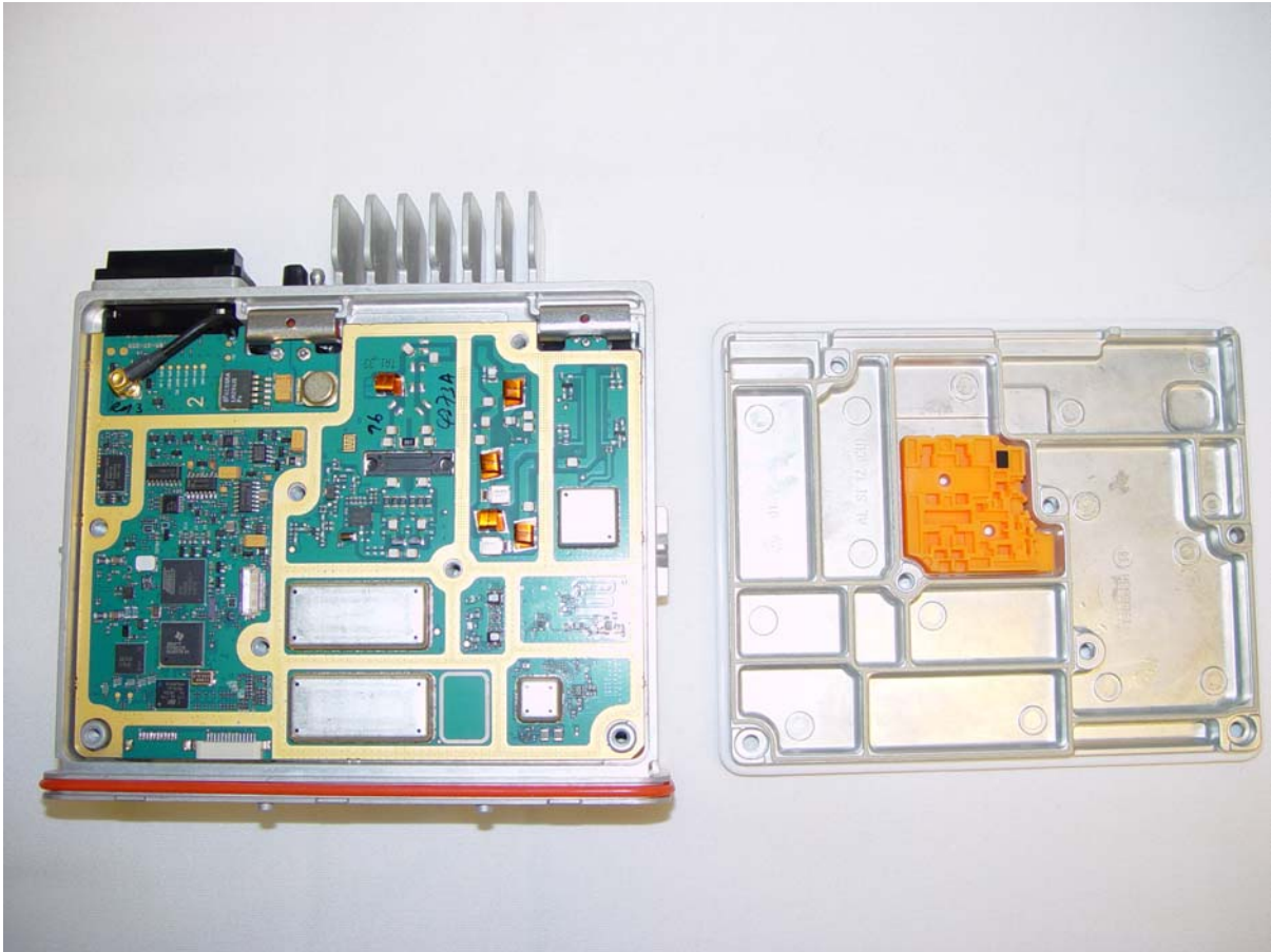
TOP VIEW OF GPS MODEL WITH CHASSIS TOP COVER REMOVED (MATING SURFACES OF TOP COVER AND CIRCUIT BOARD IN CHASSIS ARE SHOWN)
