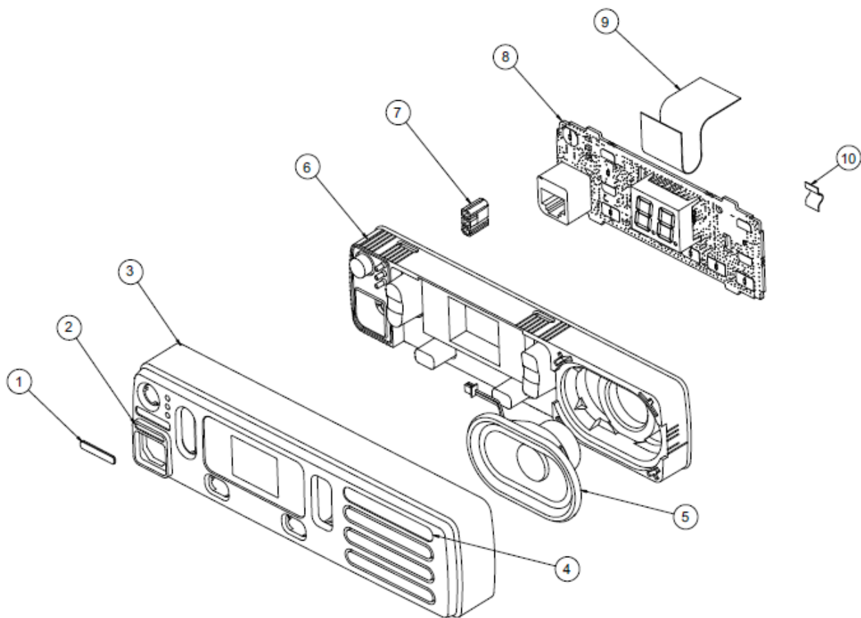
Exploded view of numeric display control head
