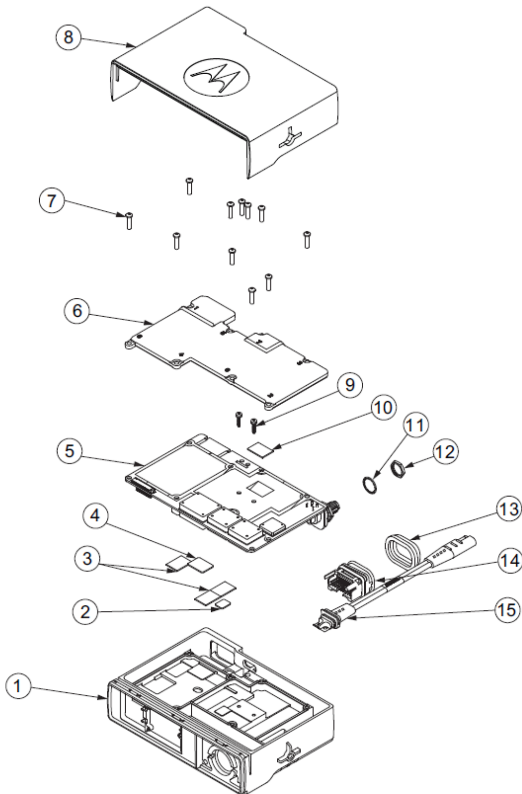
Exploded View of Radio
