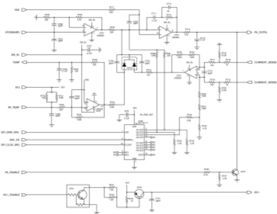
Figure 5.4 - Transmitter Power Limiting Circuit Diagram
