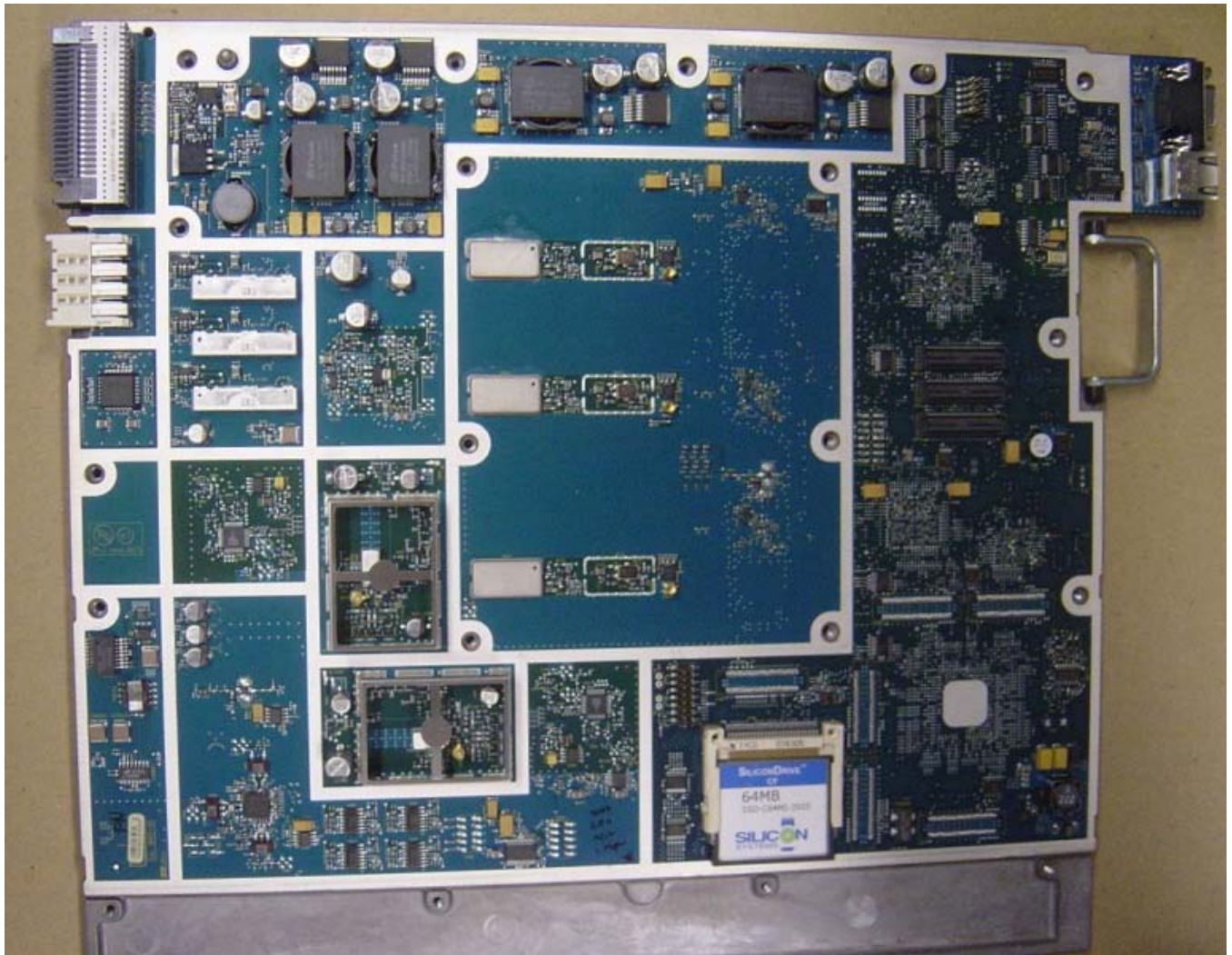
Internal Front View – Transceiver Module Circuit Board Top View
