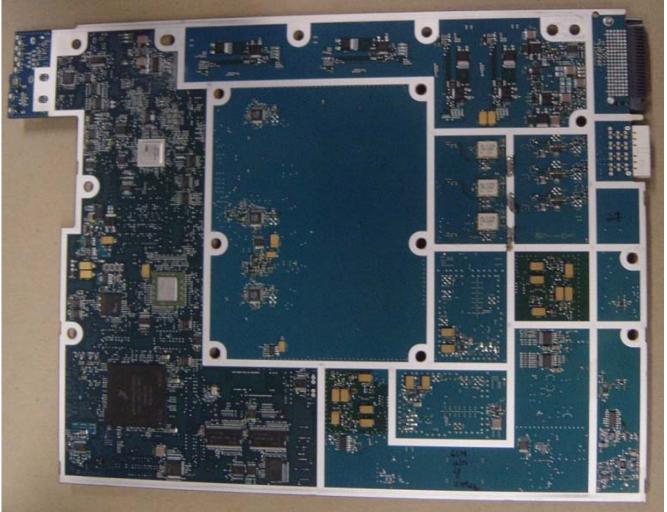
Internal Back View – Transceiver Module
