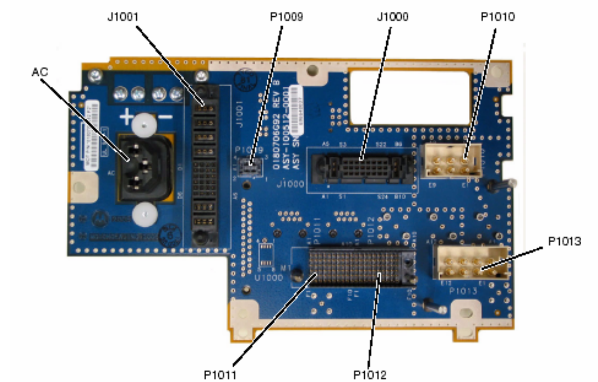
Internal Front View – Backplane
