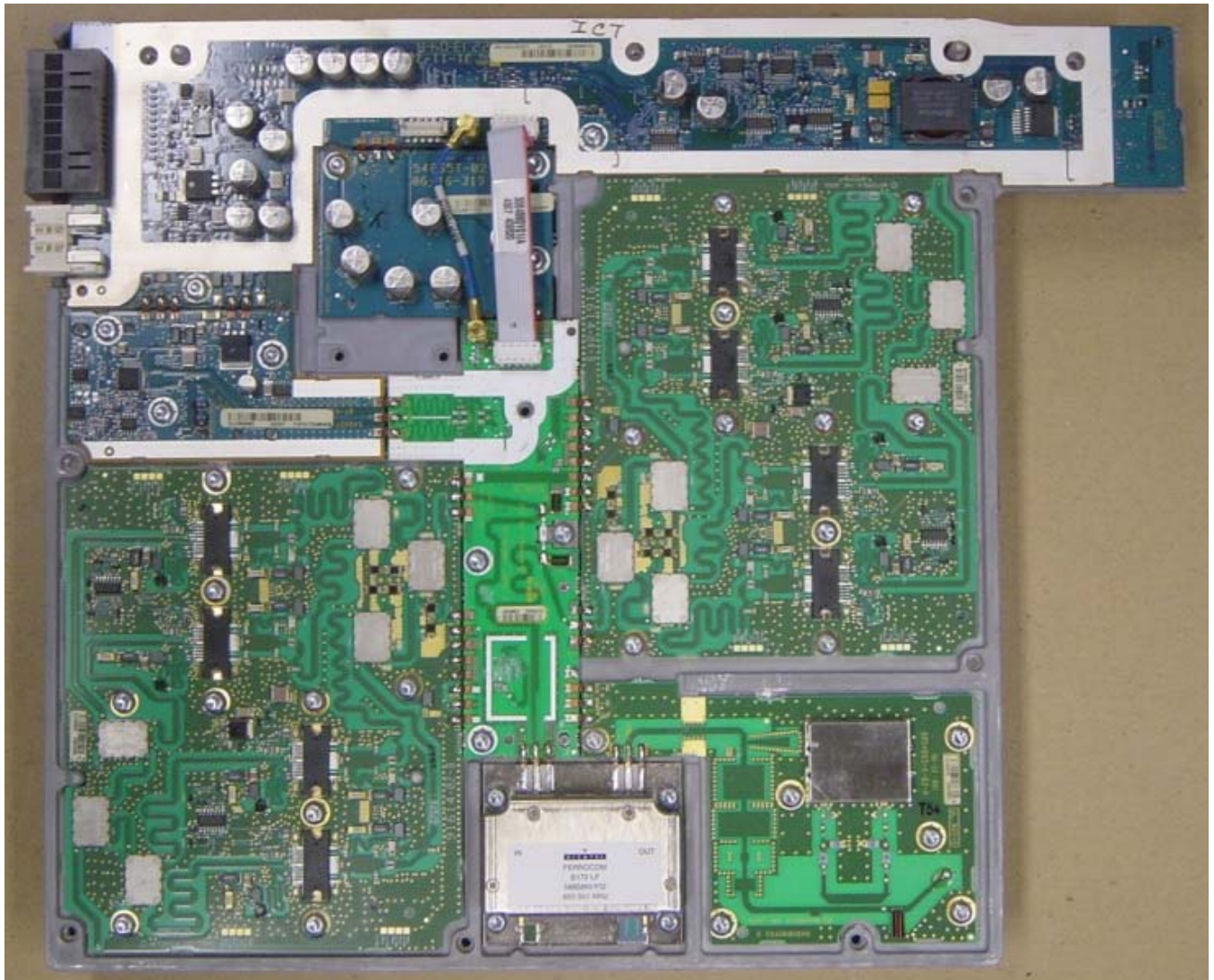
Internal Front View – Power Amplifier Module, Cover Removed
